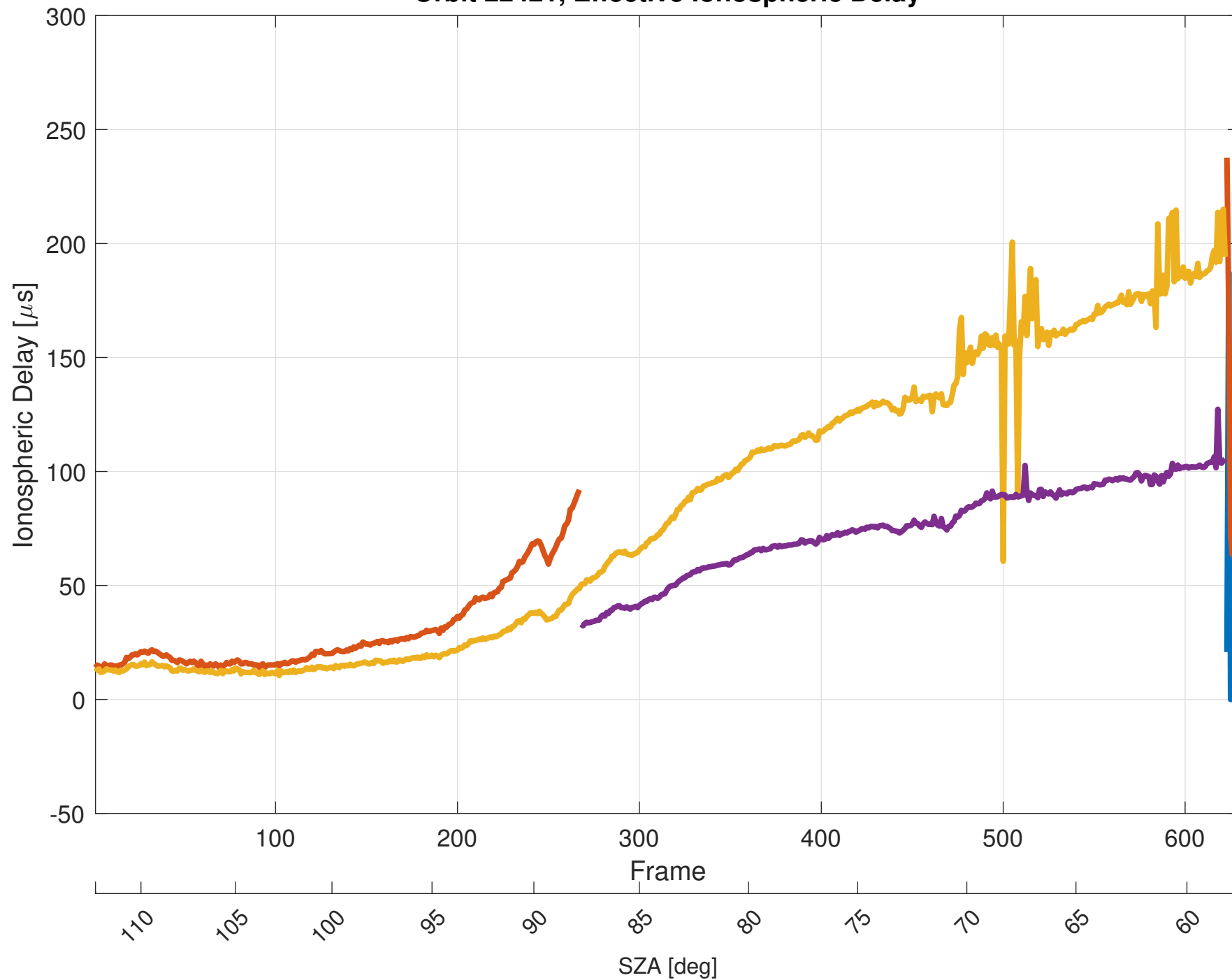
Orbit 22421, Effective Ionospheric Delay
