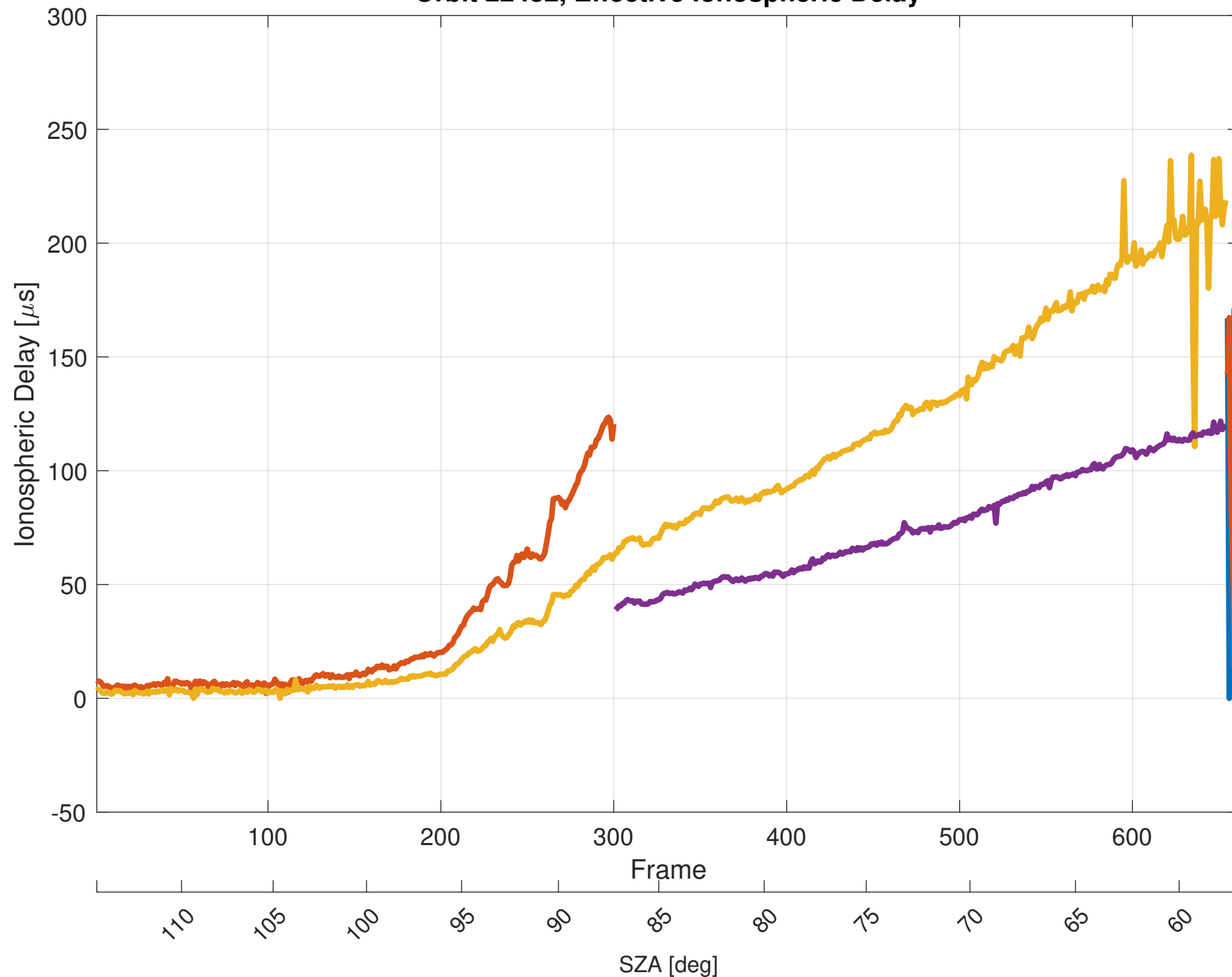
Orbit 22432, Effective Ionospheric Delay
