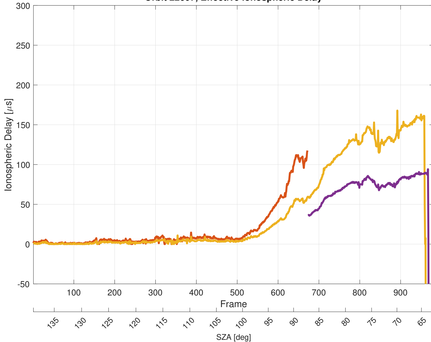
Orbit 22607, Effective Ionospheric Delay
