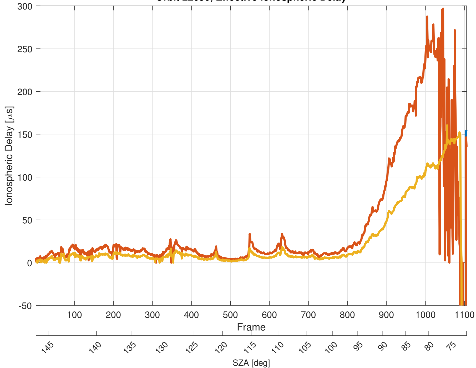
Orbit 22650, Effective Ionospheric Delay
