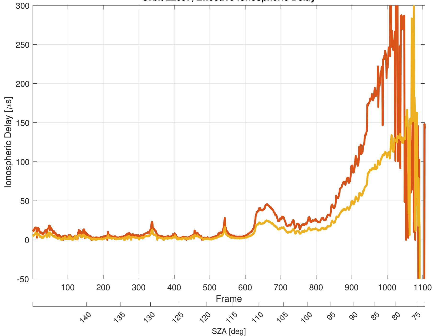
Orbit 22657, Effective Ionospheric Delay
