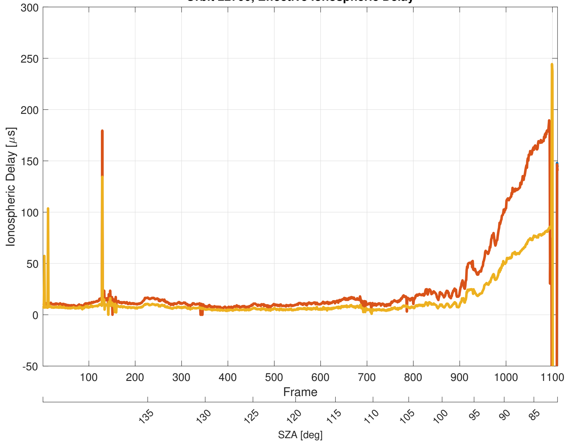
Orbit 22700, Effective Ionospheric Delay
