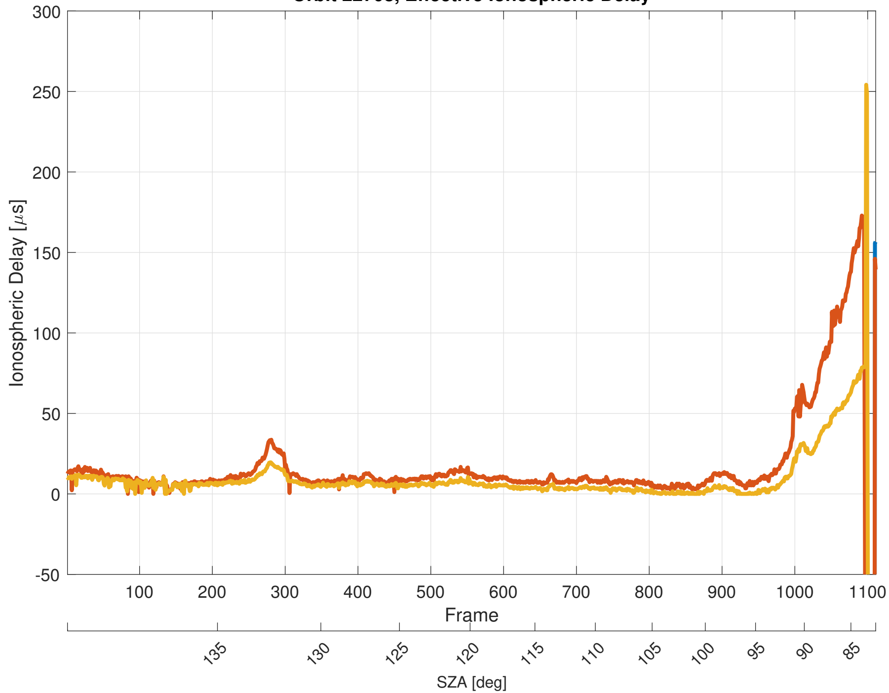
Orbit 22708, Effective Ionospheric Delay
