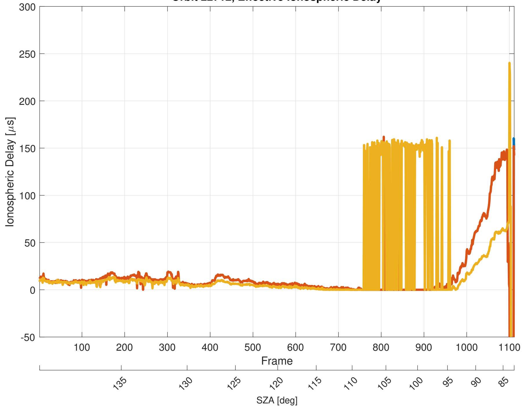
Orbit 22712, Effective Ionospheric Delay
