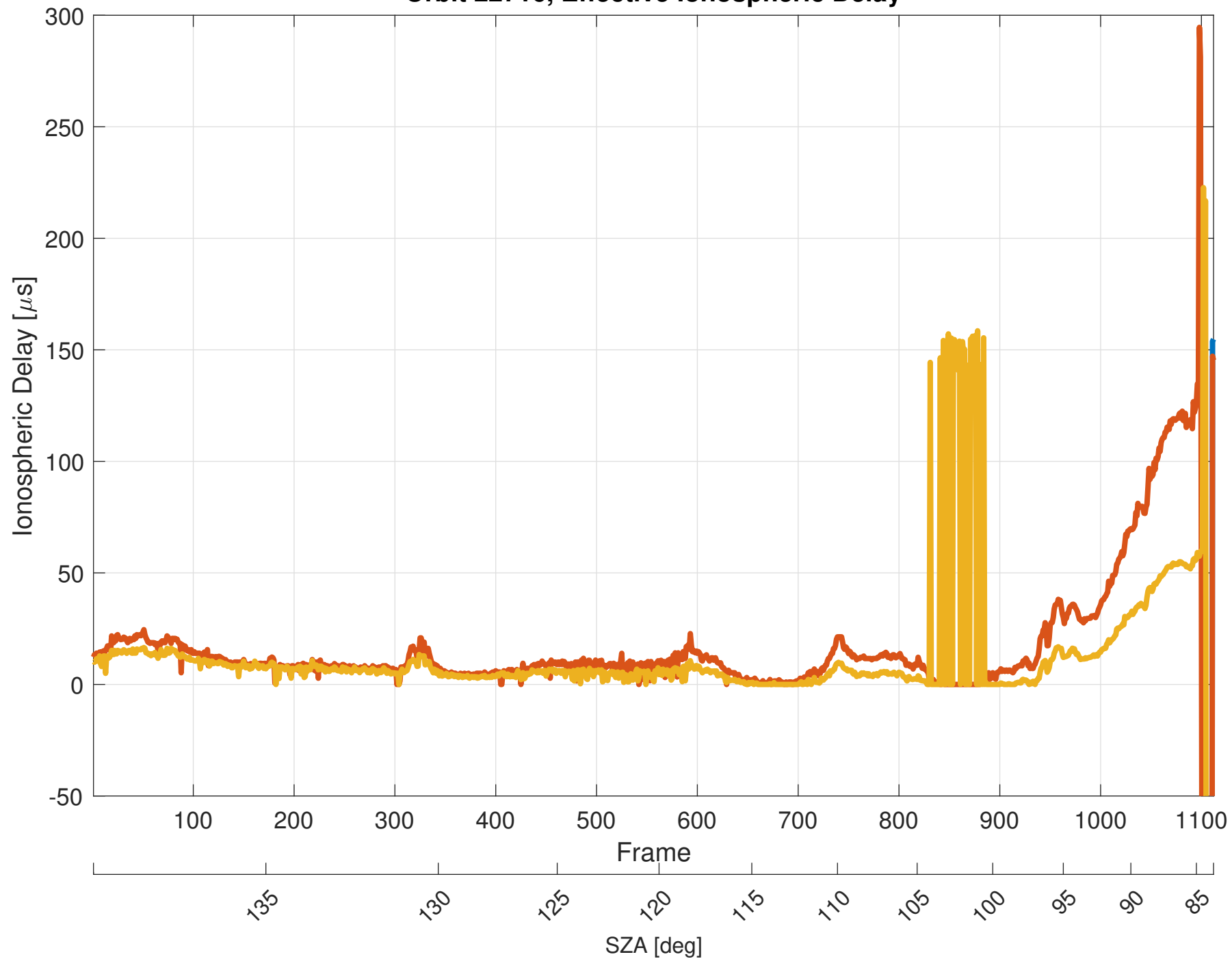
Orbit 22716, Effective Ionospheric Delay
