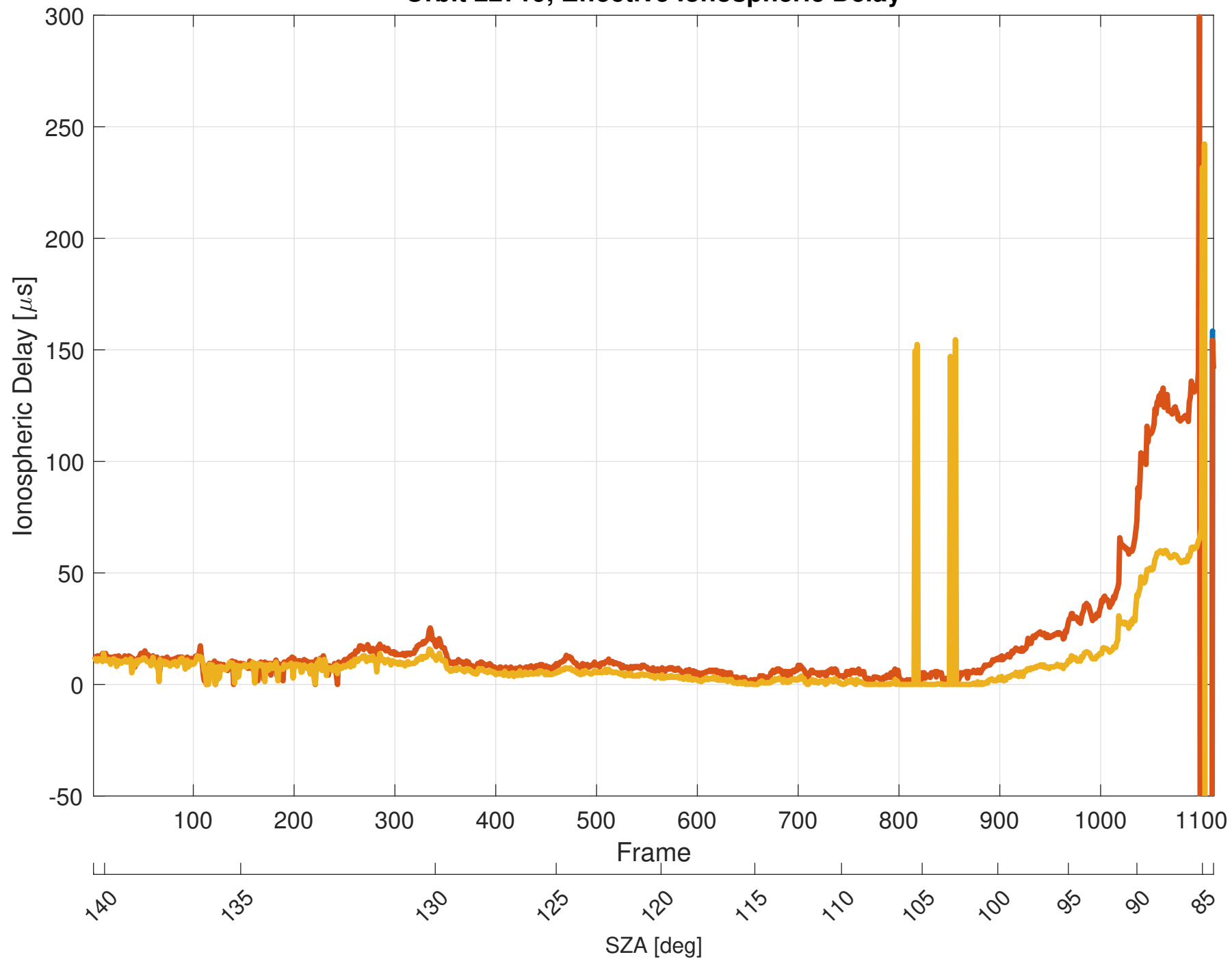
Orbit 22719, Effective Ionospheric Delay
