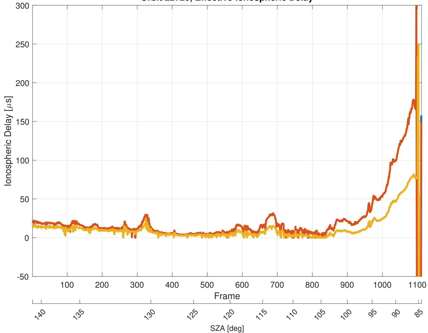
Orbit 22720, Effective Ionospheric Delay
