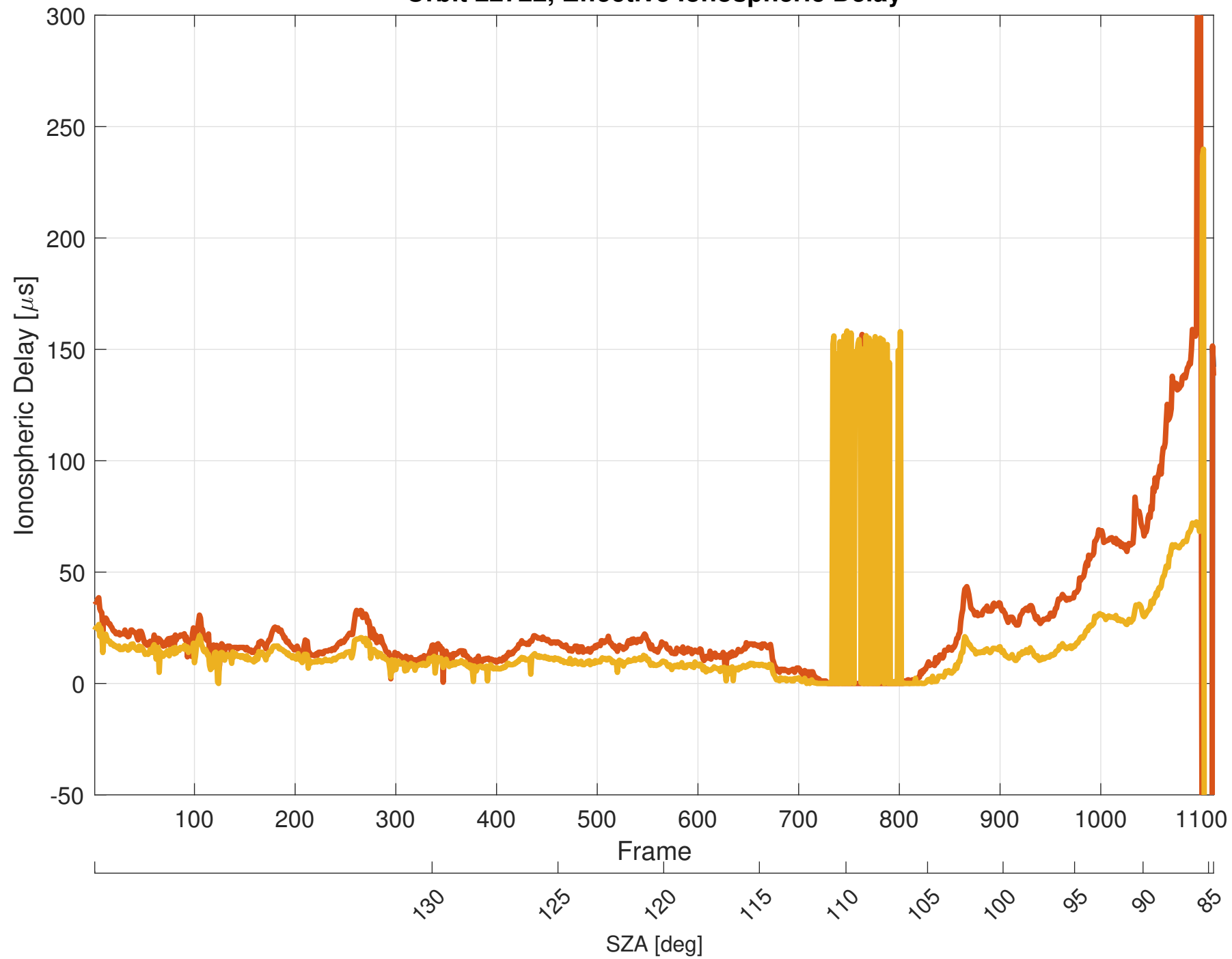
Orbit 22722, Effective Ionospheric Delay
