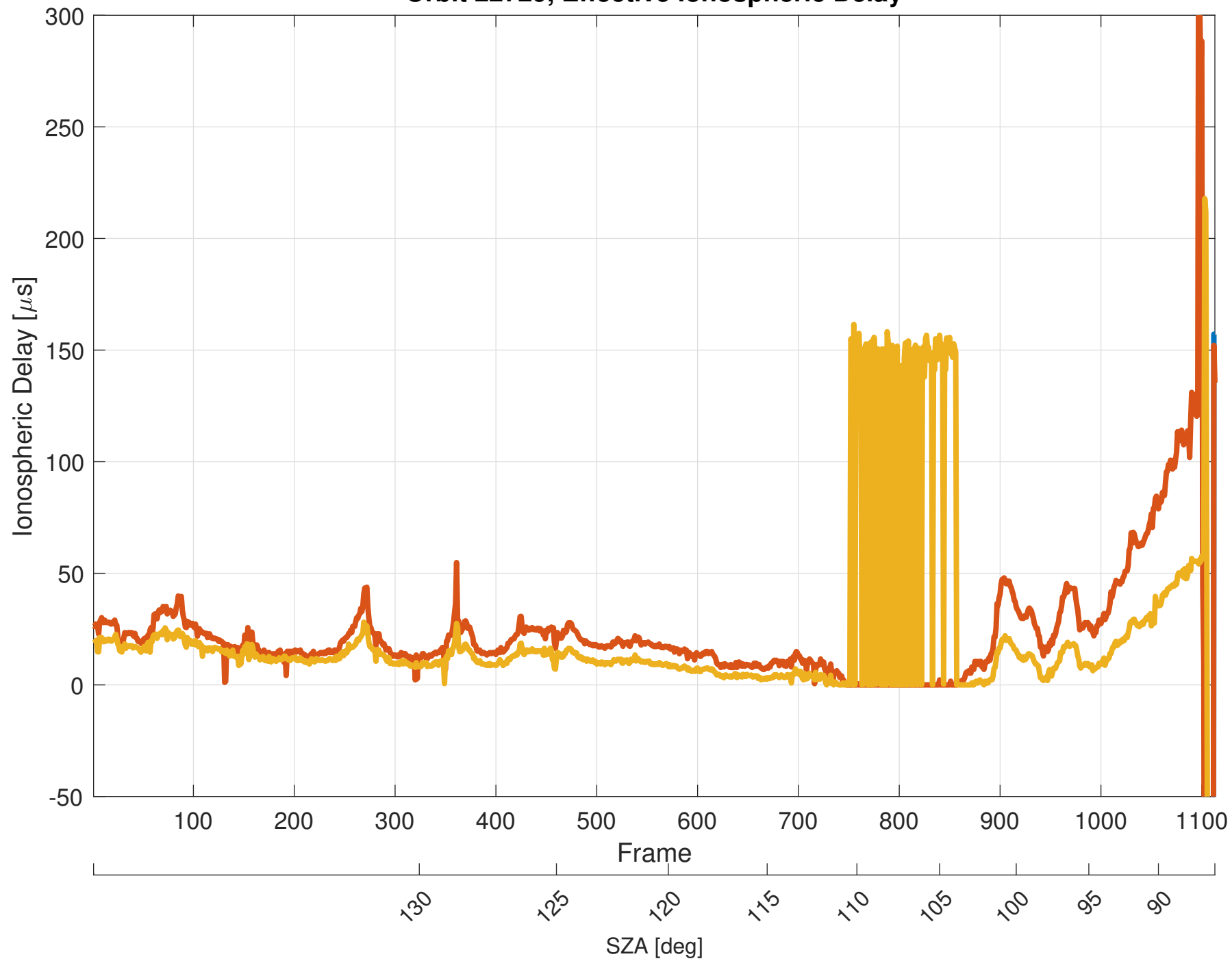
Orbit 22729, Effective Ionospheric Delay
