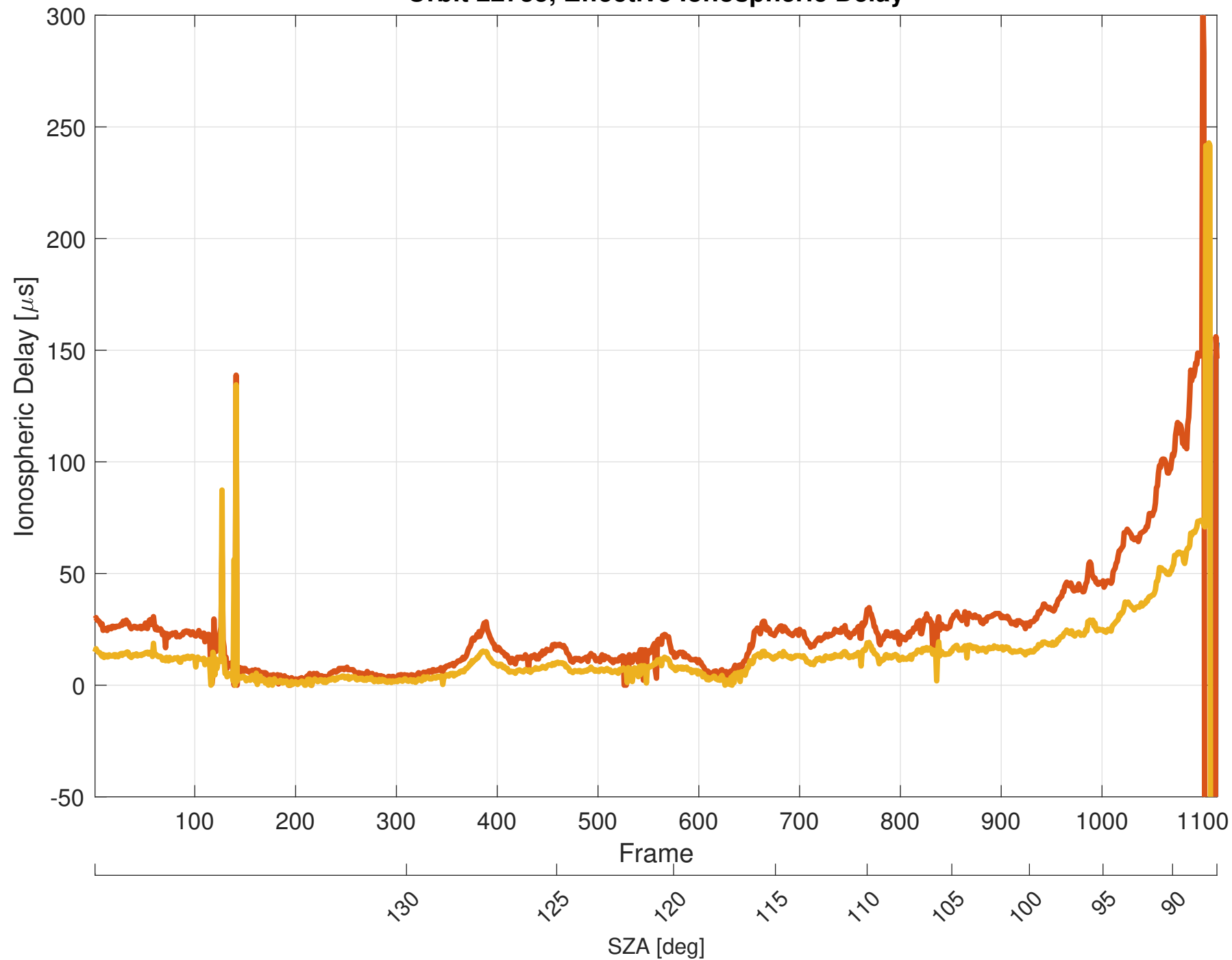
Orbit 22735, Effective Ionospheric Delay
