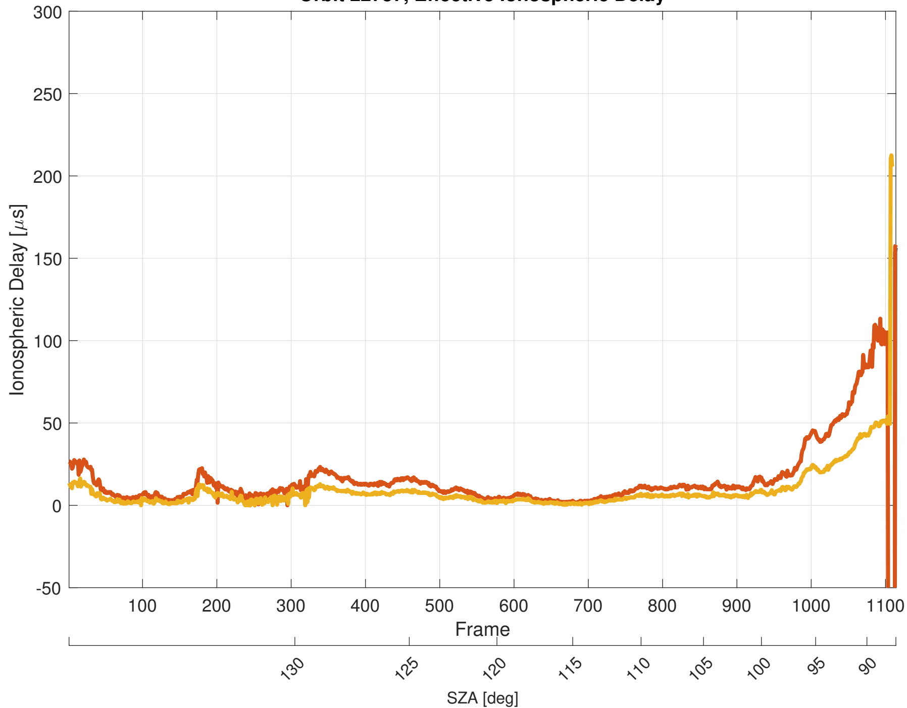
Orbit 22737, Effective Ionospheric Delay
