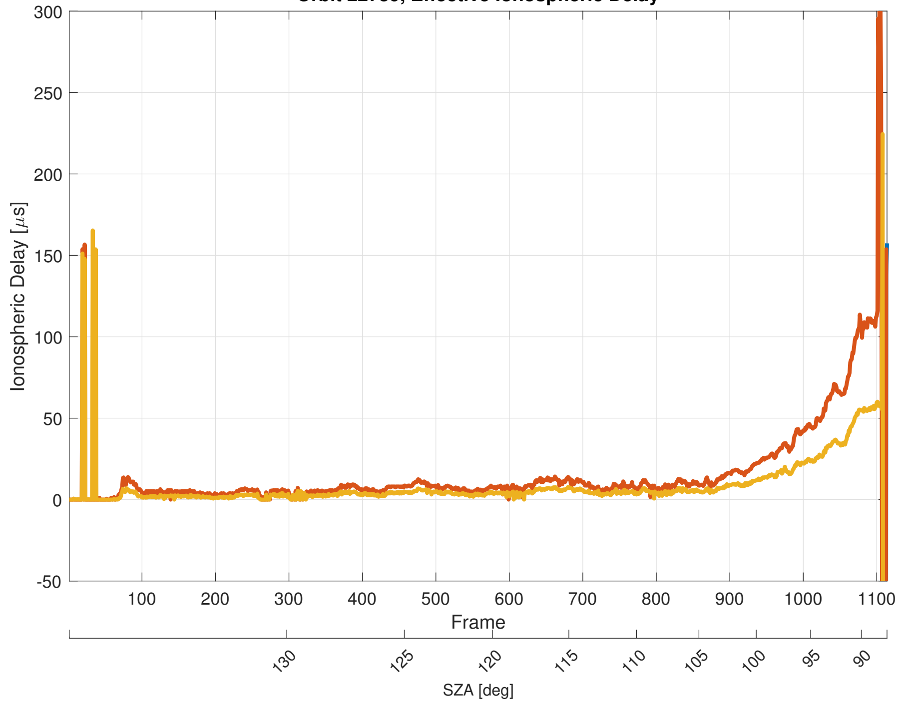
Orbit 22739, Effective Ionospheric Delay
