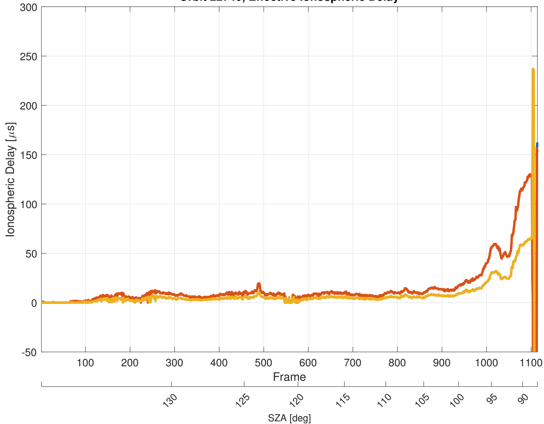
Orbit 22740, Effective Ionospheric Delay
