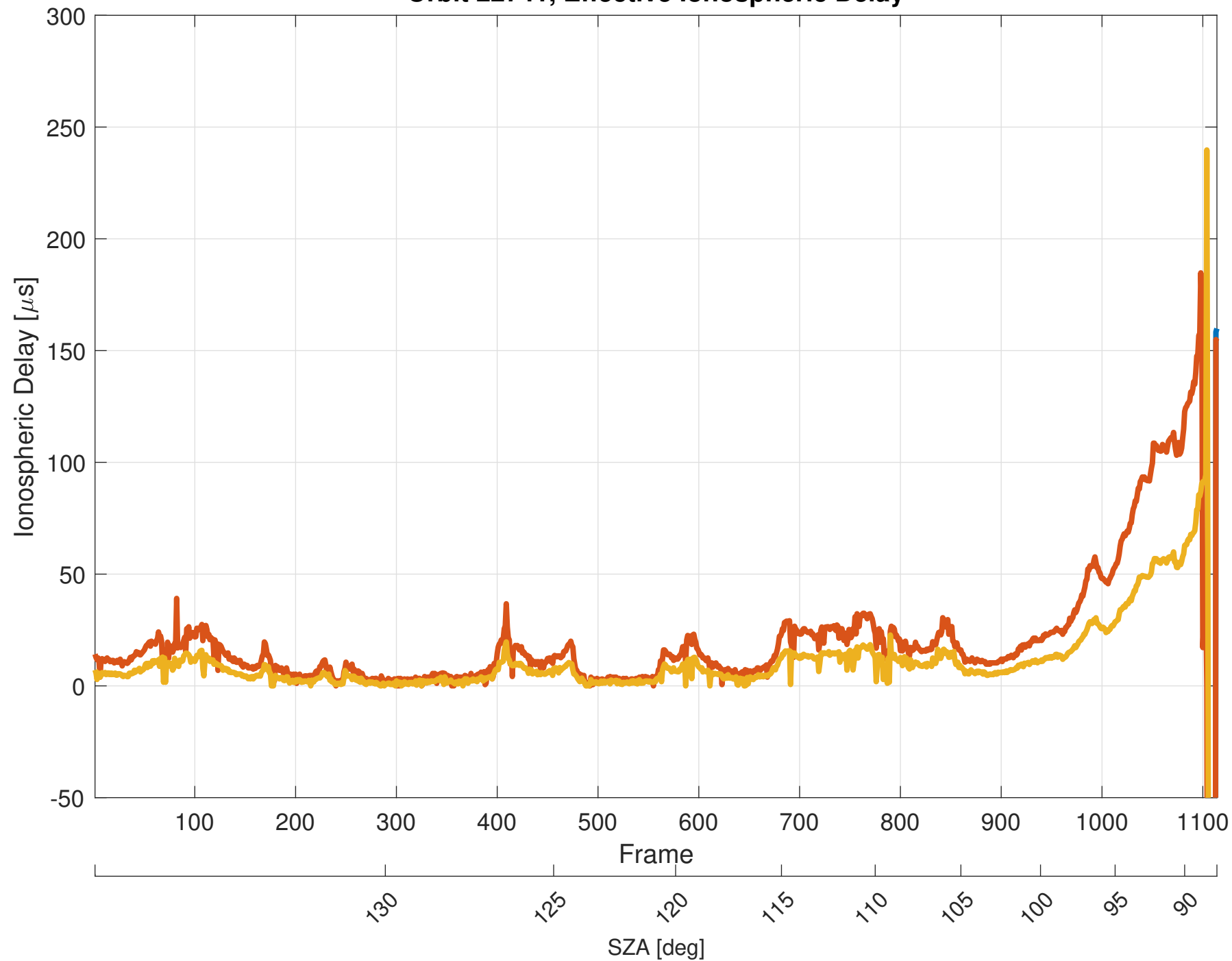
Orbit 22741, Effective Ionospheric Delay
