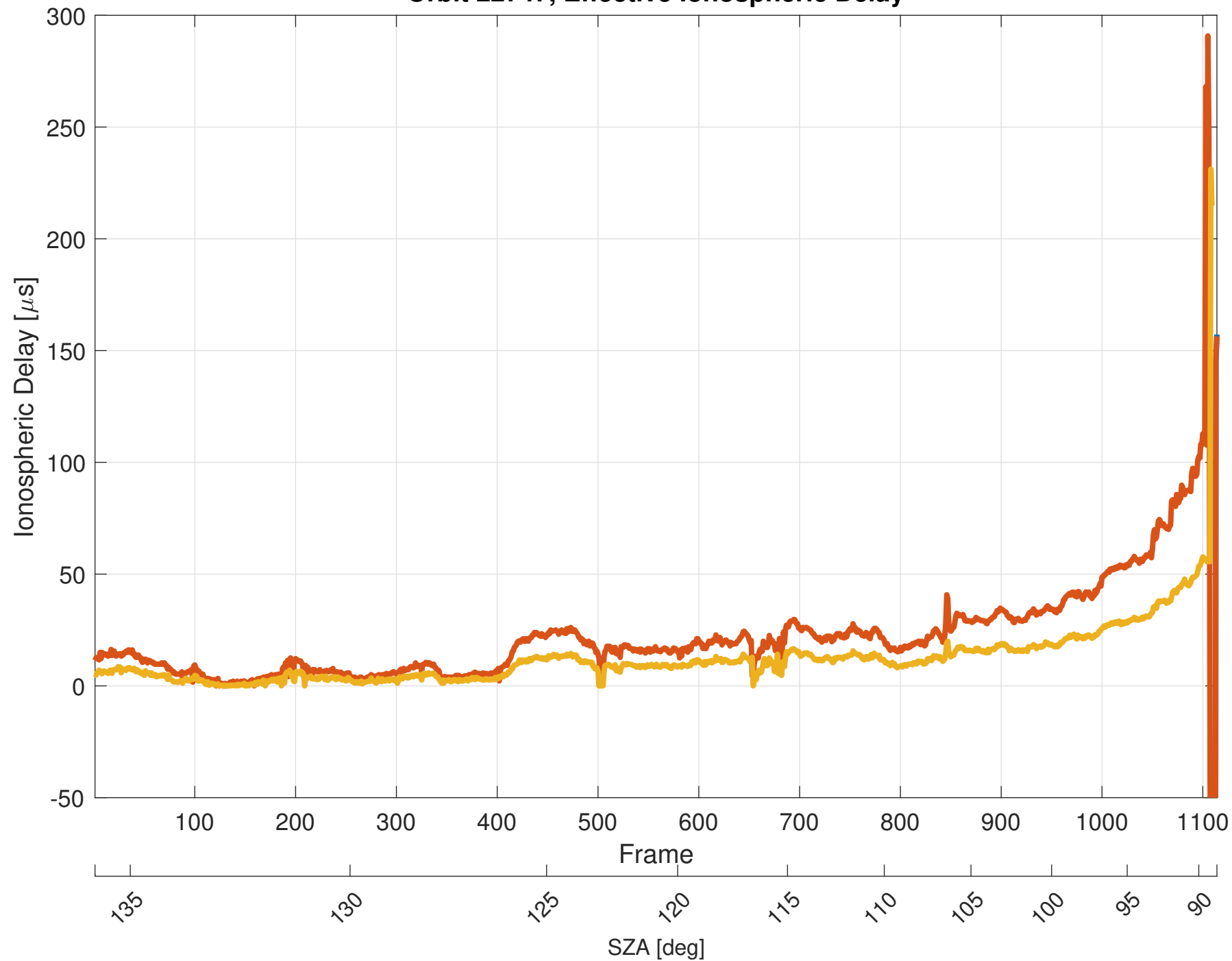
Orbit 22747, Effective Ionospheric Delay
