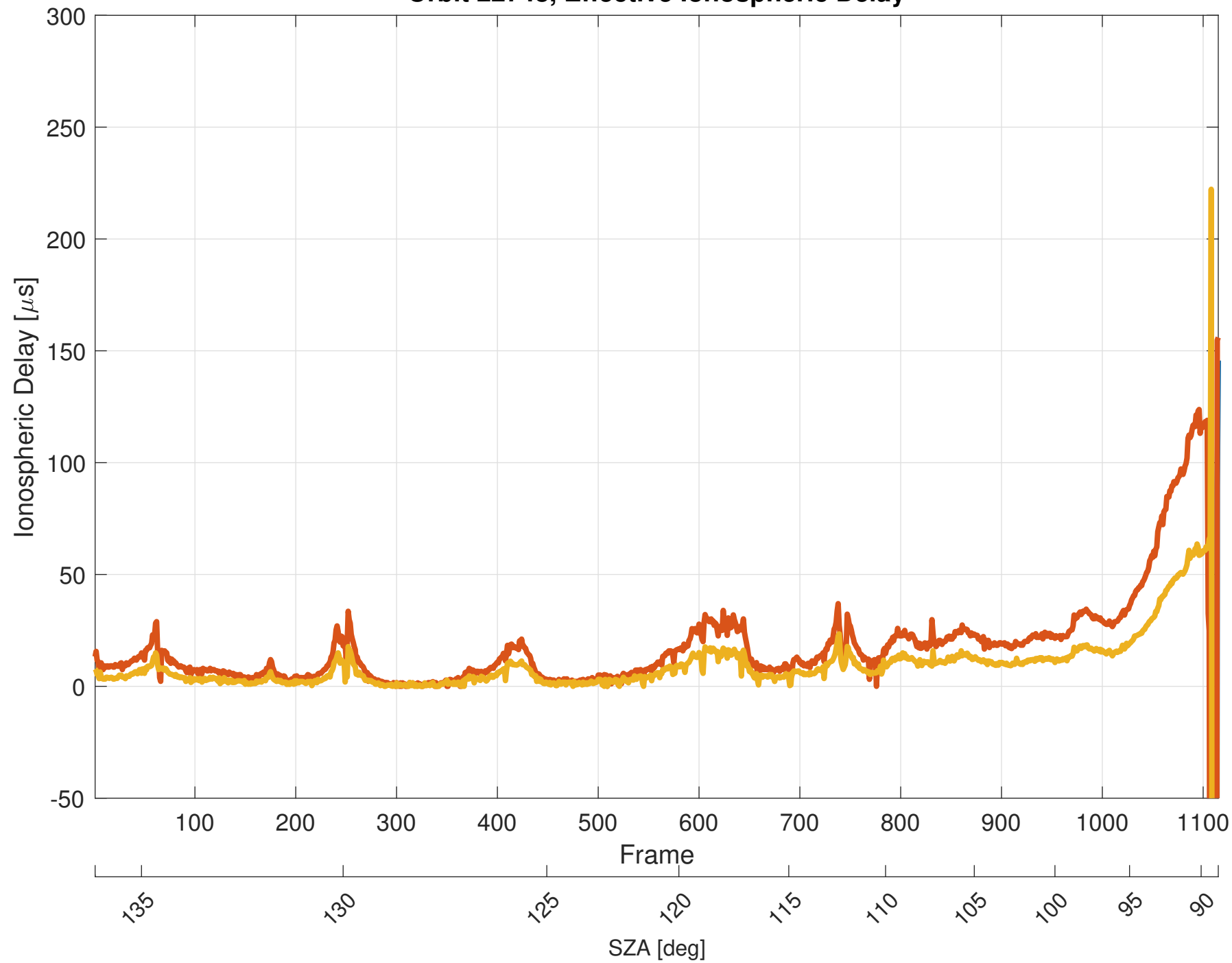
Orbit 22748, Effective Ionospheric Delay
