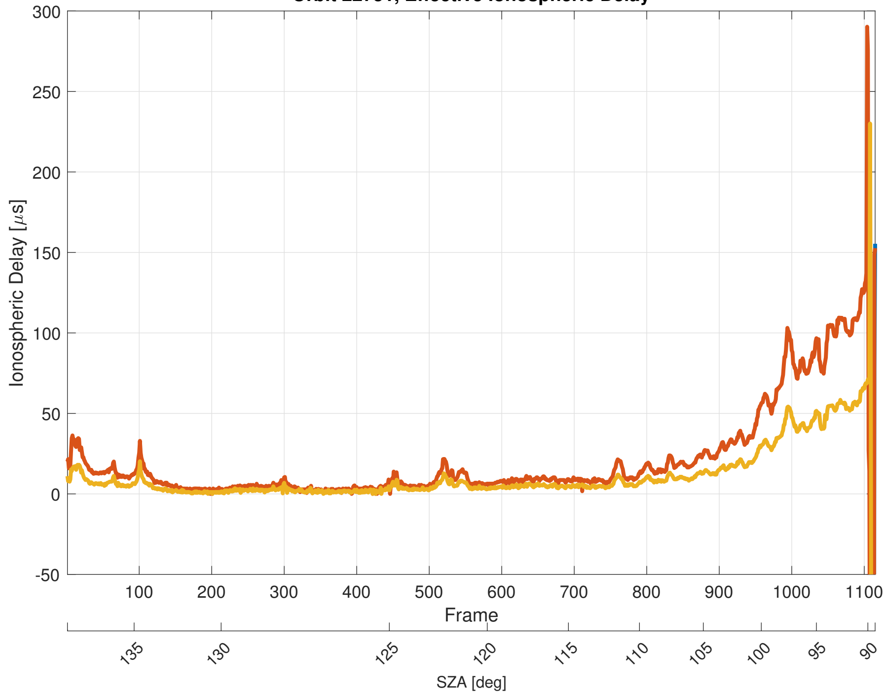
Orbit 22751, Effective Ionospheric Delay
