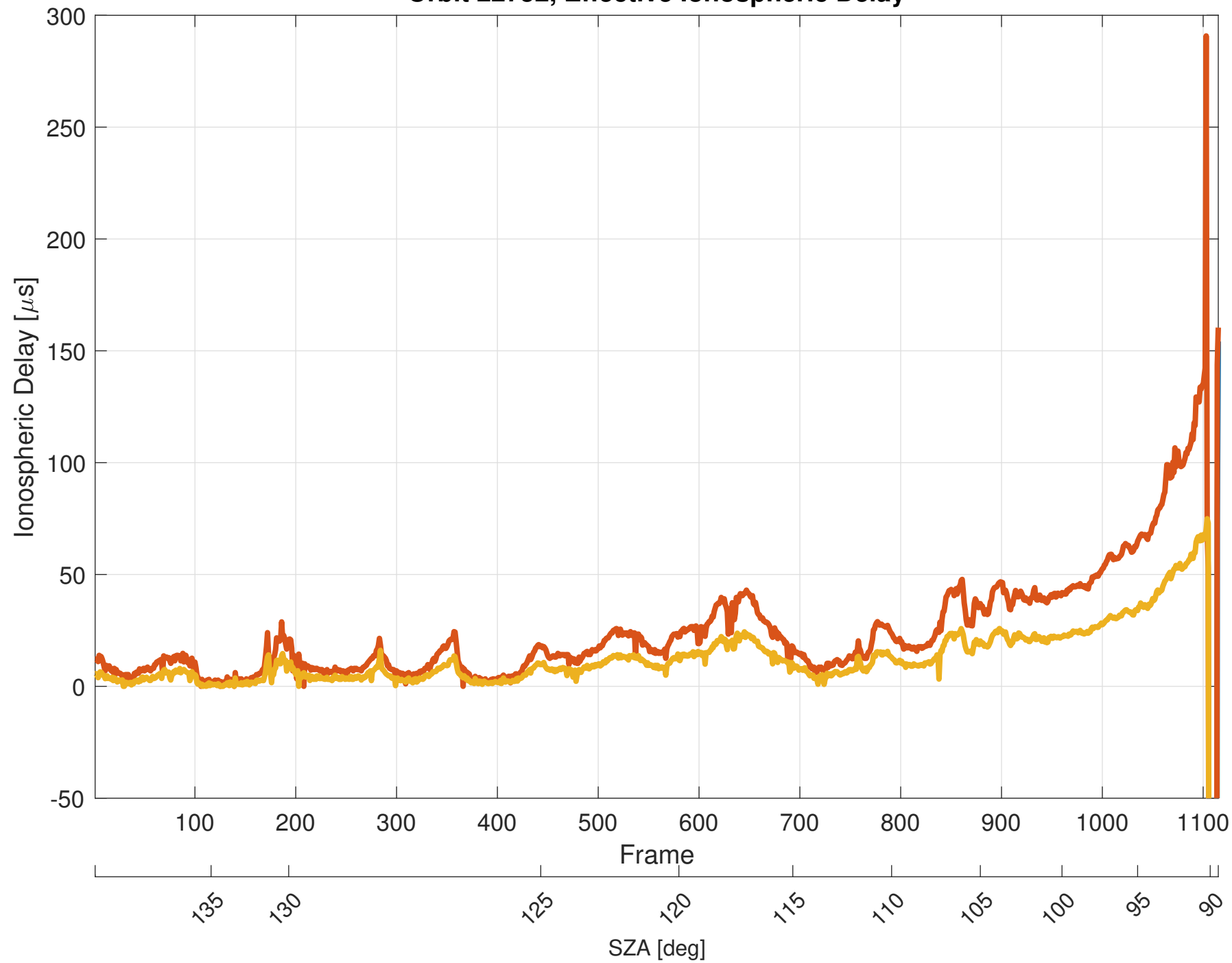
Orbit 22752, Effective Ionospheric Delay
