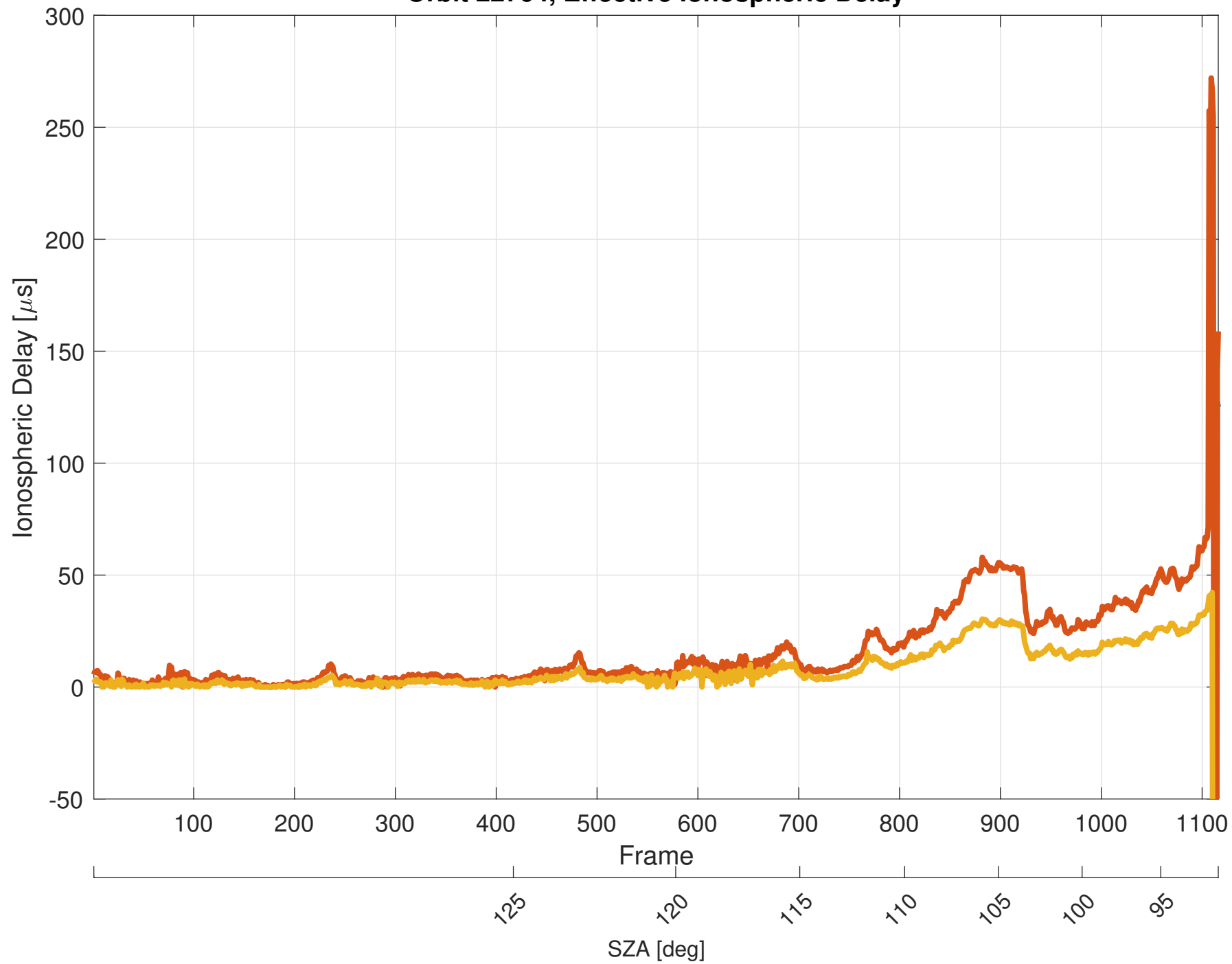
Orbit 22764, Effective Ionospheric Delay
