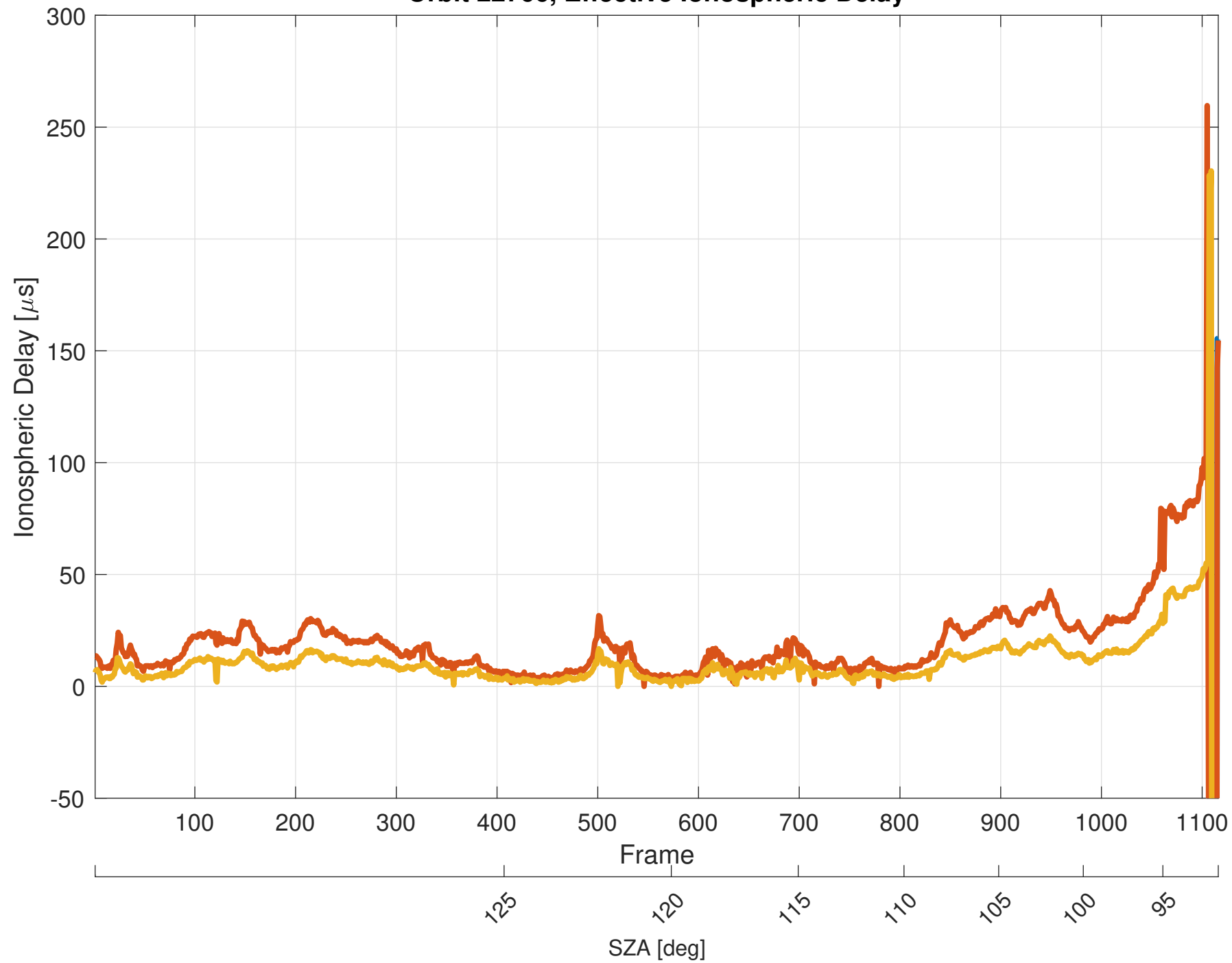
Orbit 22766, Effective Ionospheric Delay
