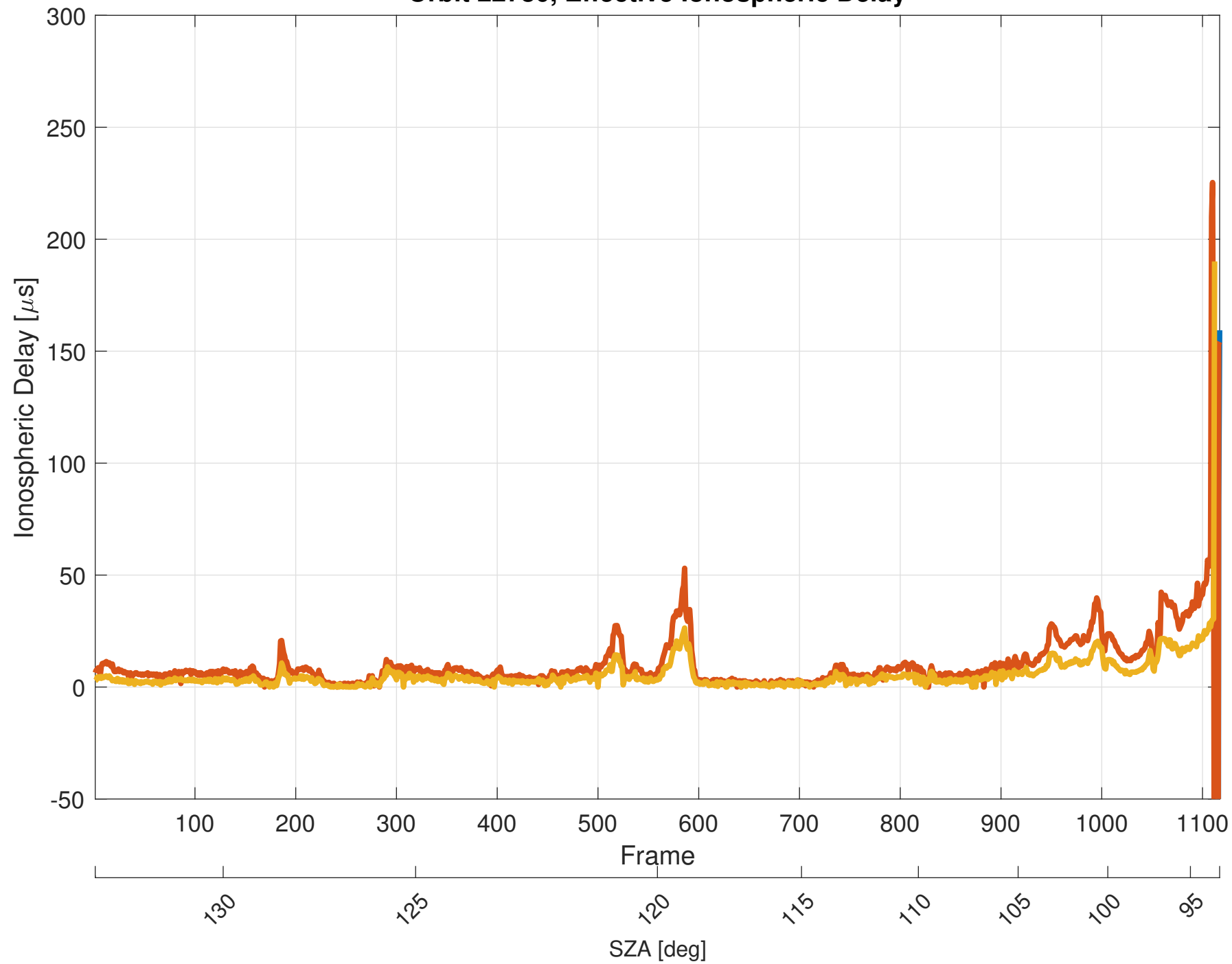
Orbit 22780, Effective Ionospheric Delay
