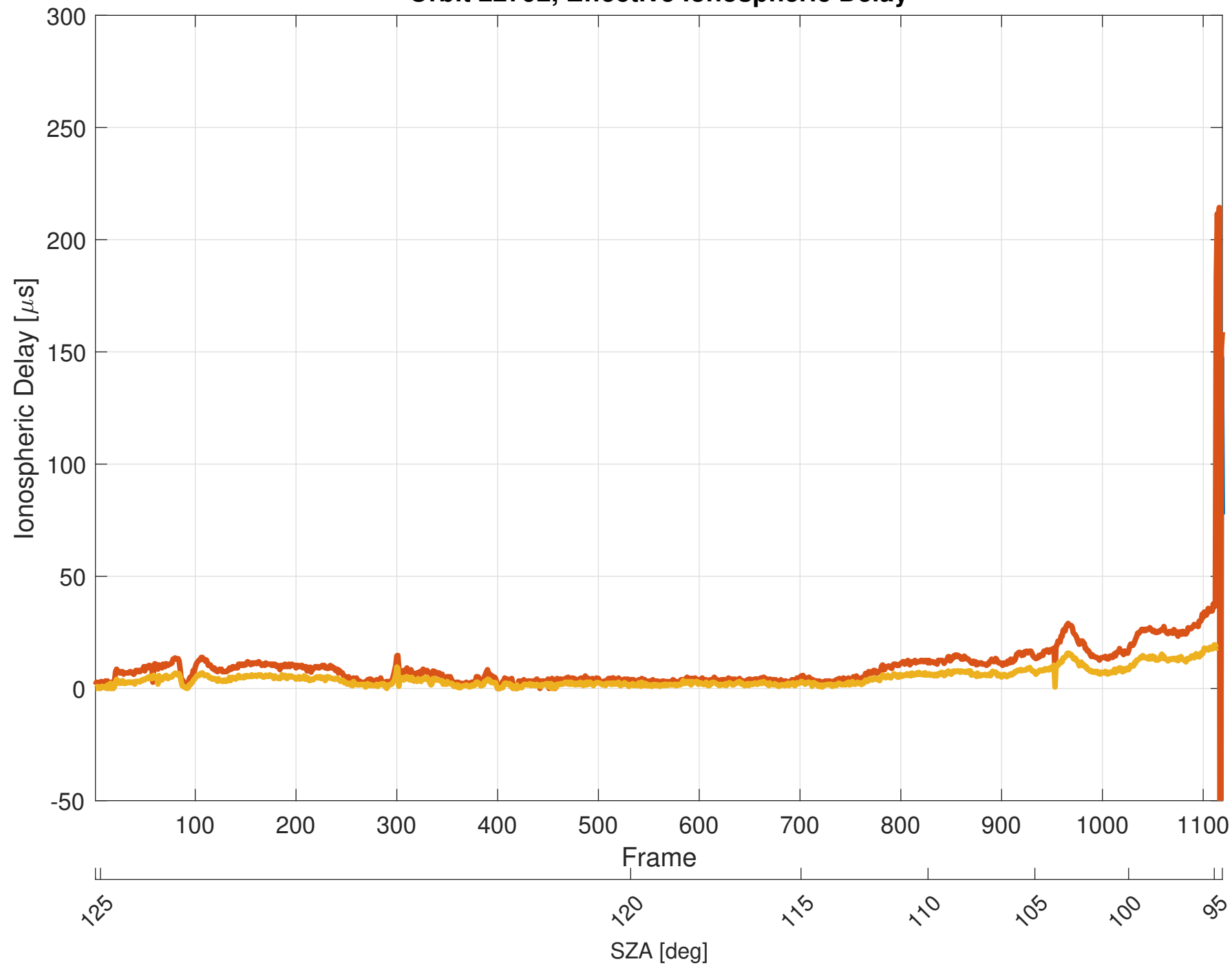
Orbit 22792, Effective Ionospheric Delay
