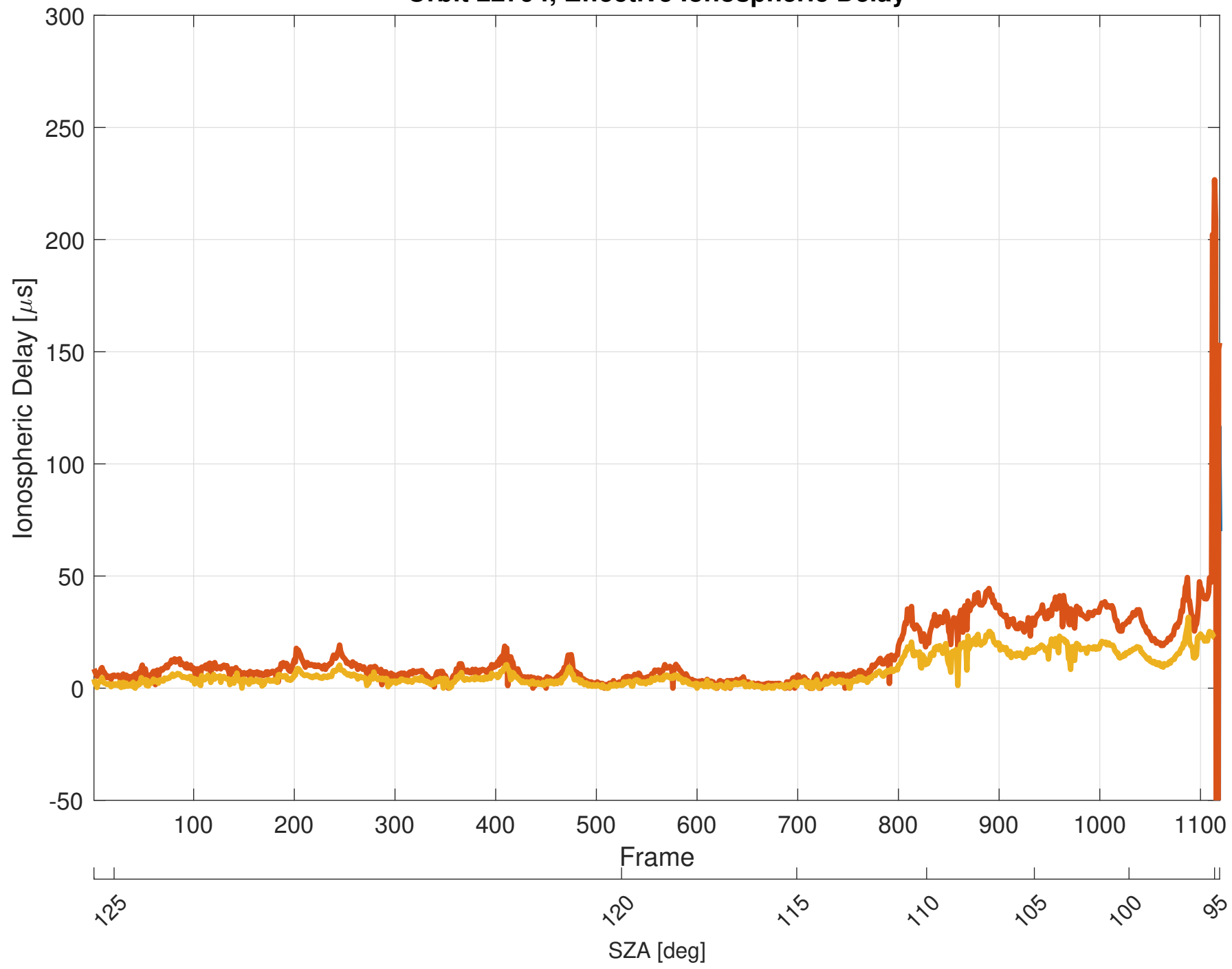
Orbit 22794, Effective Ionospheric Delay
