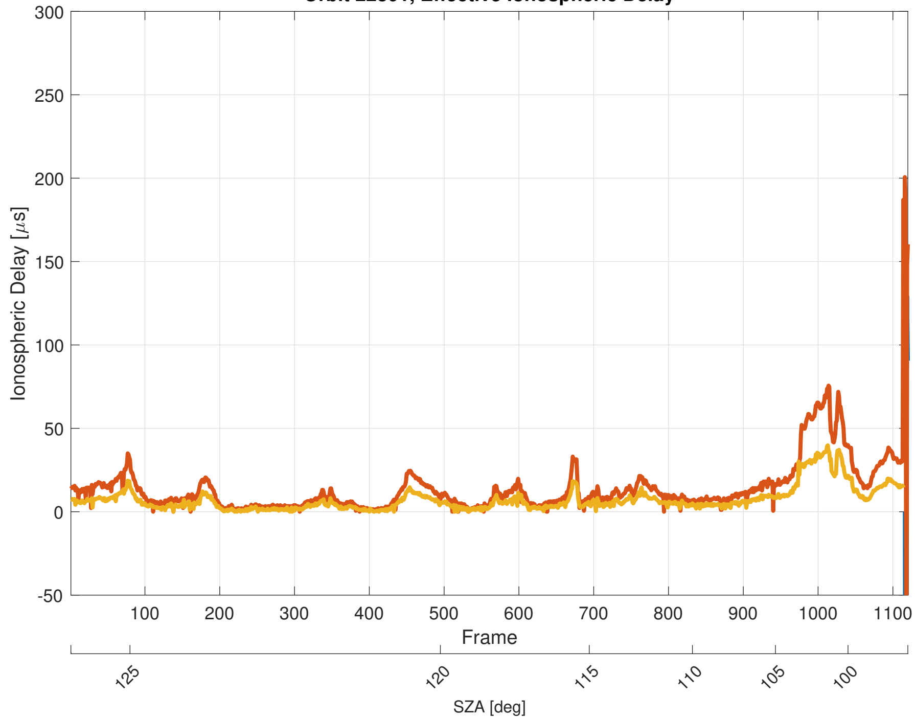
Orbit 22801, Effective Ionospheric Delay
