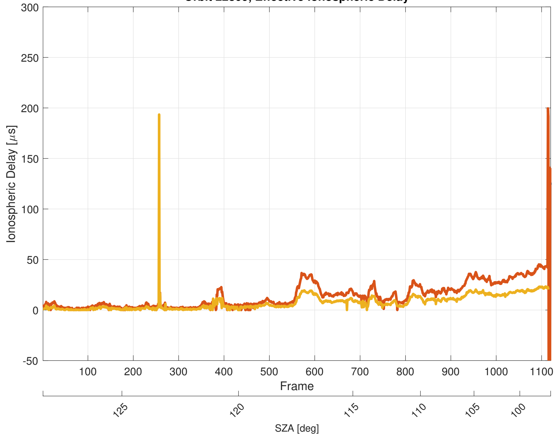
Orbit 22809, Effective Ionospheric Delay
