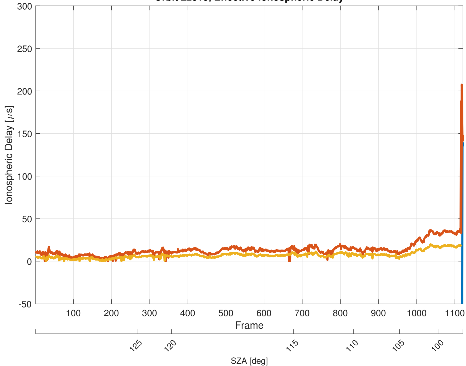
Orbit 22813, Effective Ionospheric Delay
