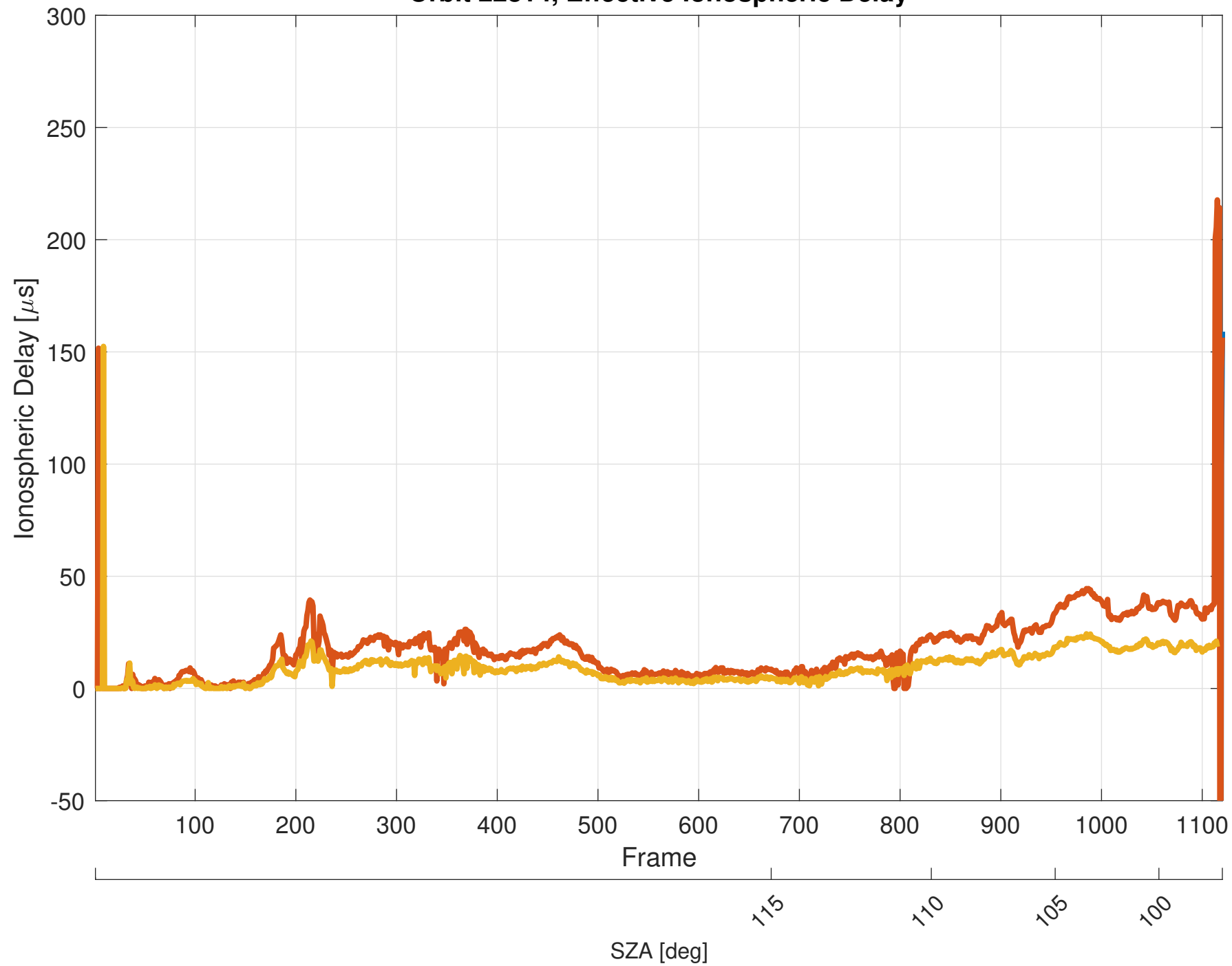
Orbit 22814, Effective Ionospheric Delay
