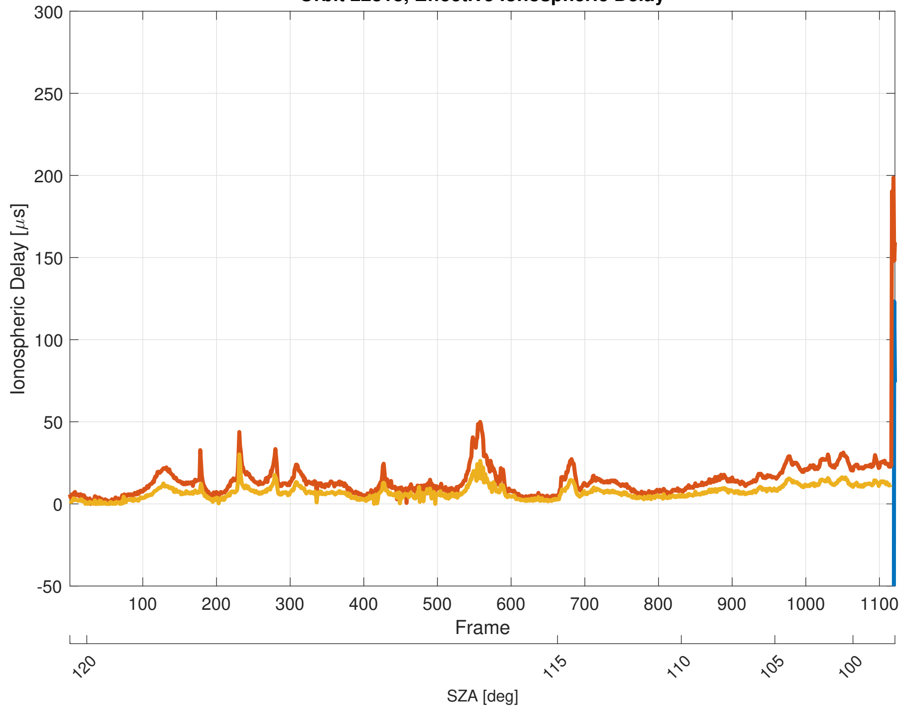
Orbit 22818, Effective Ionospheric Delay
