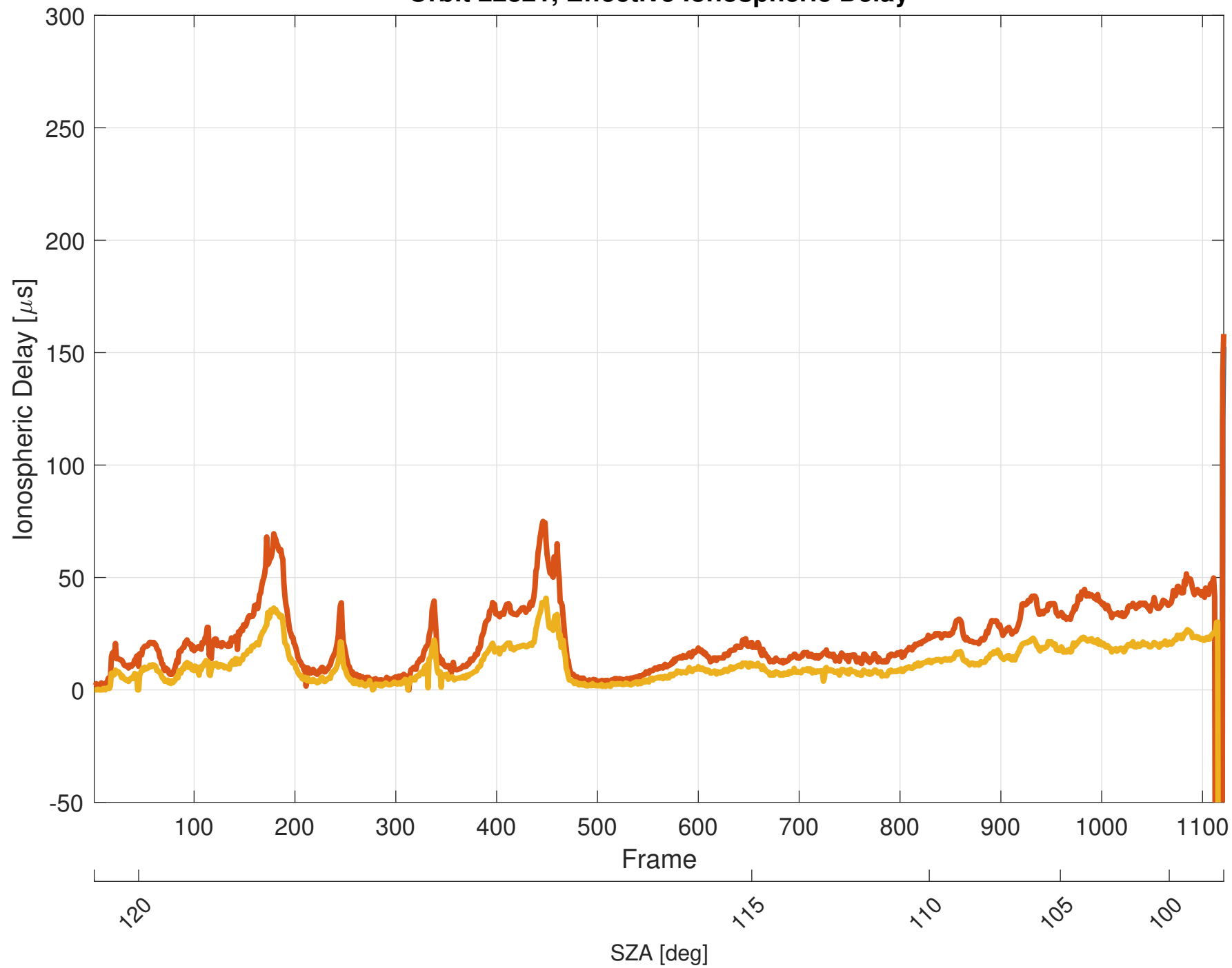
Orbit 22821, Effective Ionospheric Delay
