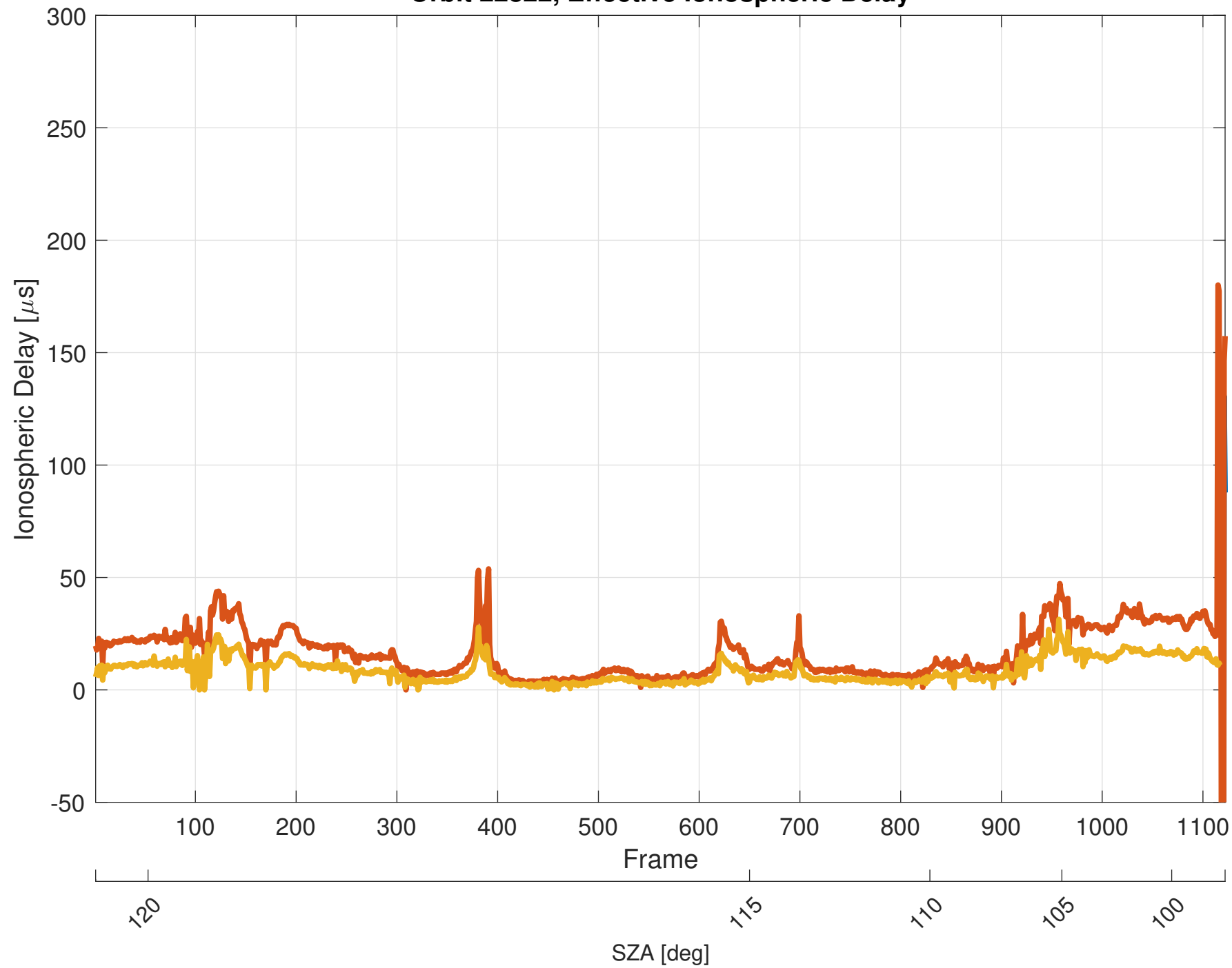
Orbit 22822, Effective Ionospheric Delay
