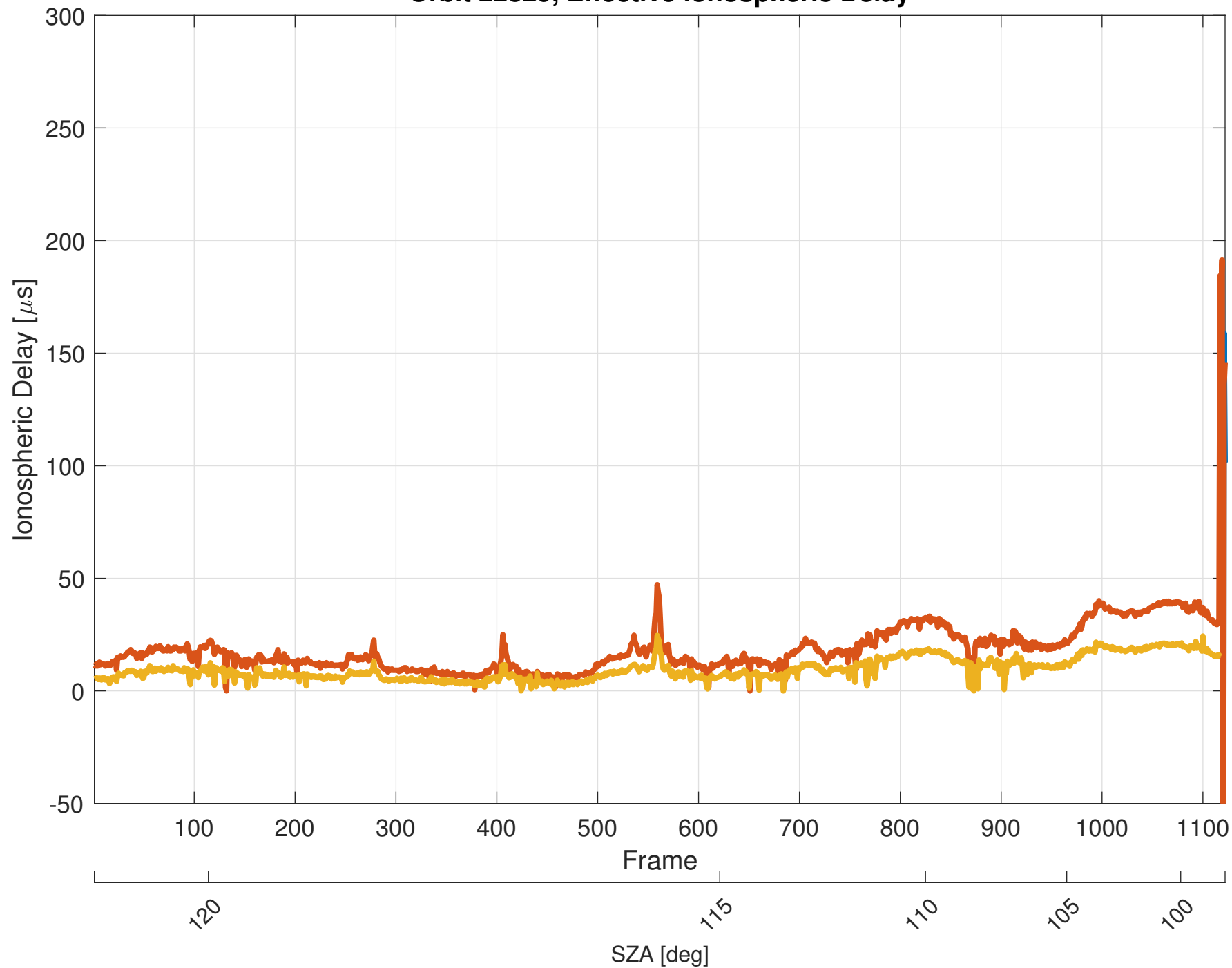
Orbit 22829, Effective Ionospheric Delay
