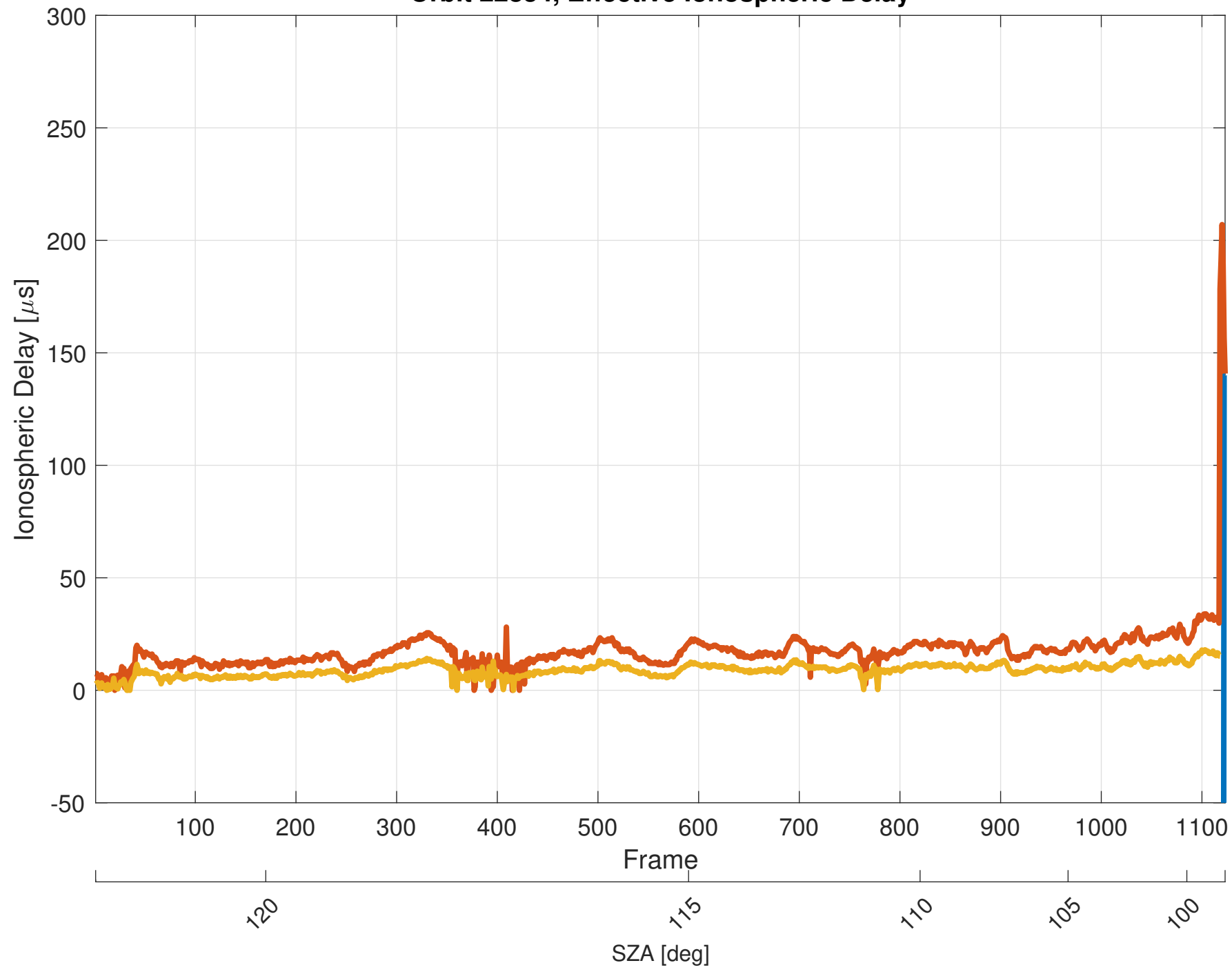
Orbit 22834, Effective Ionospheric Delay
