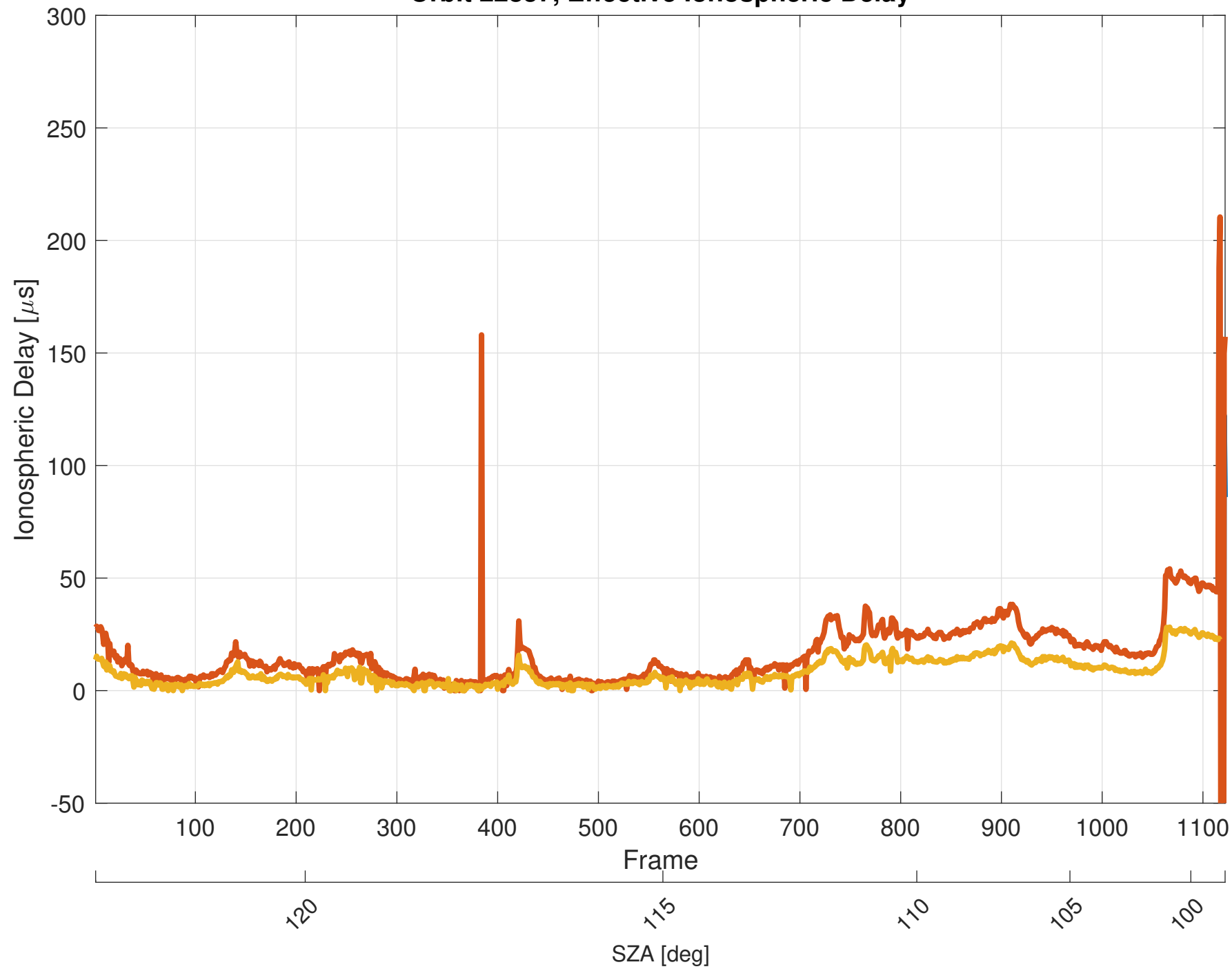
Orbit 22837, Effective Ionospheric Delay
