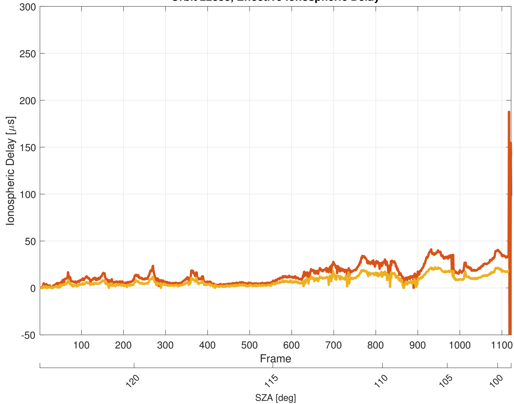
Orbit 22838, Effective Ionospheric Delay
