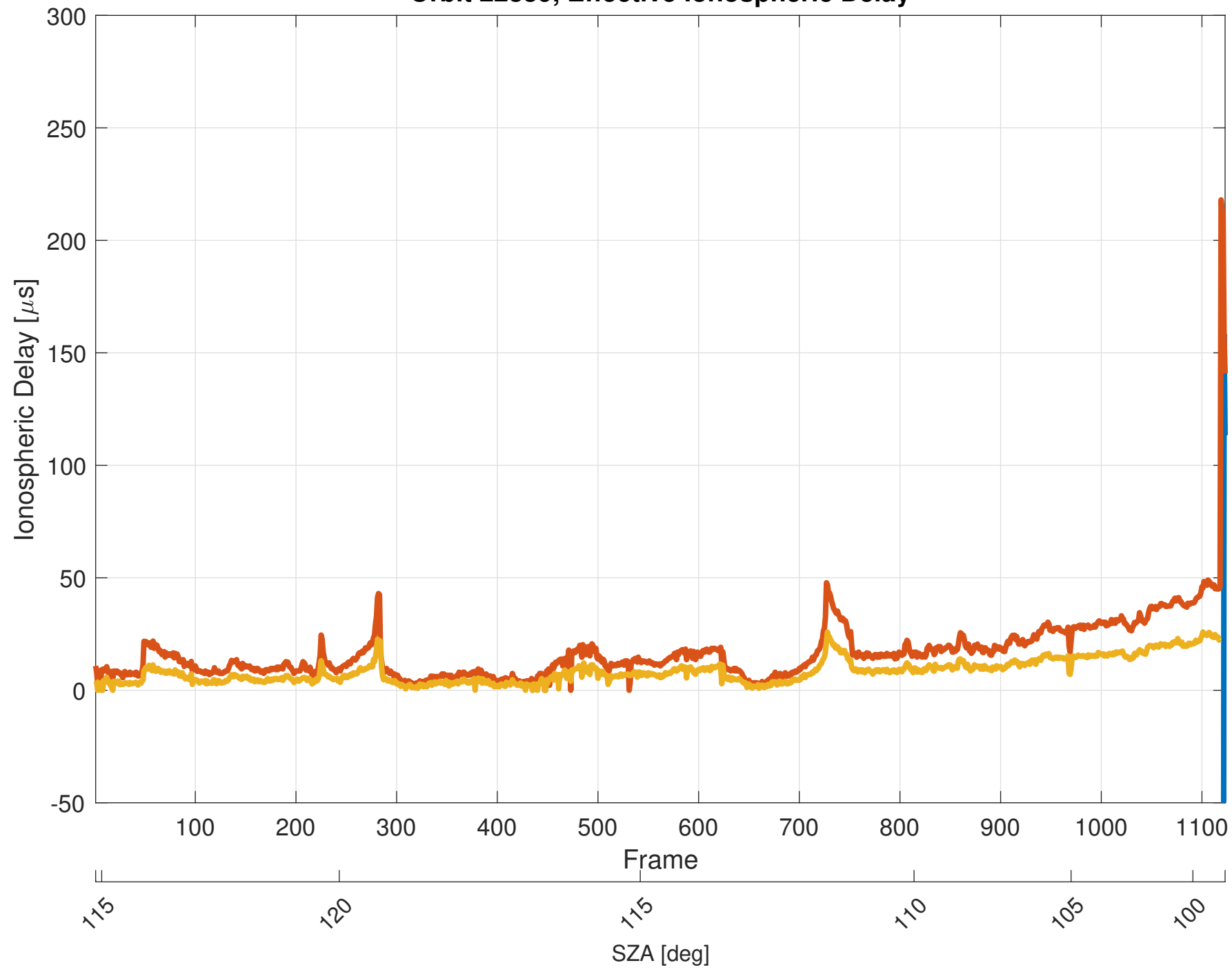
Orbit 22839, Effective Ionospheric Delay
