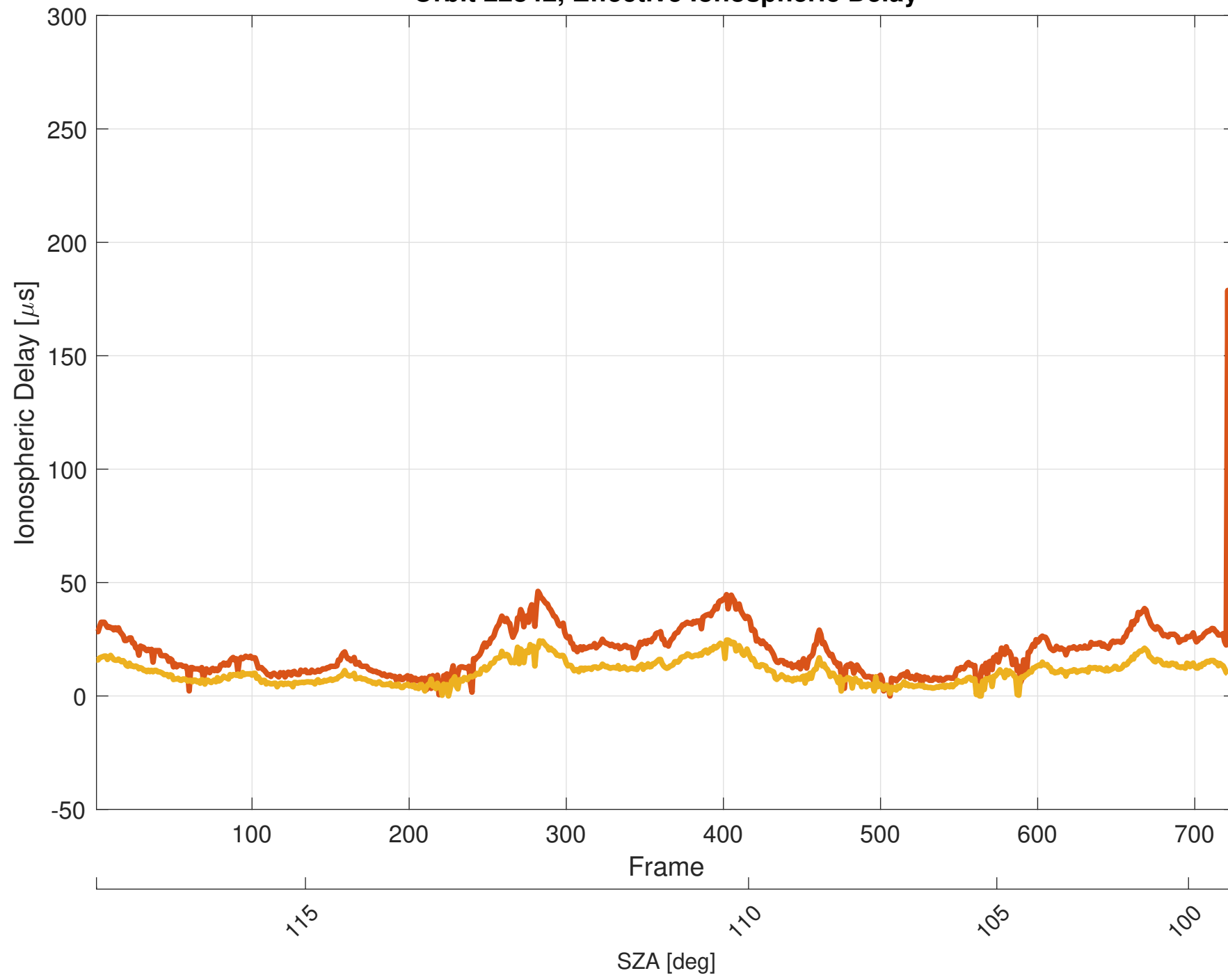
Orbit 22842, Effective Ionospheric Delay
