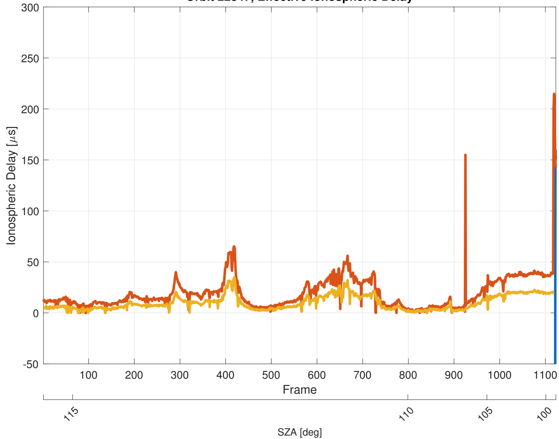
Orbit 22847, Effective Ionospheric Delay
