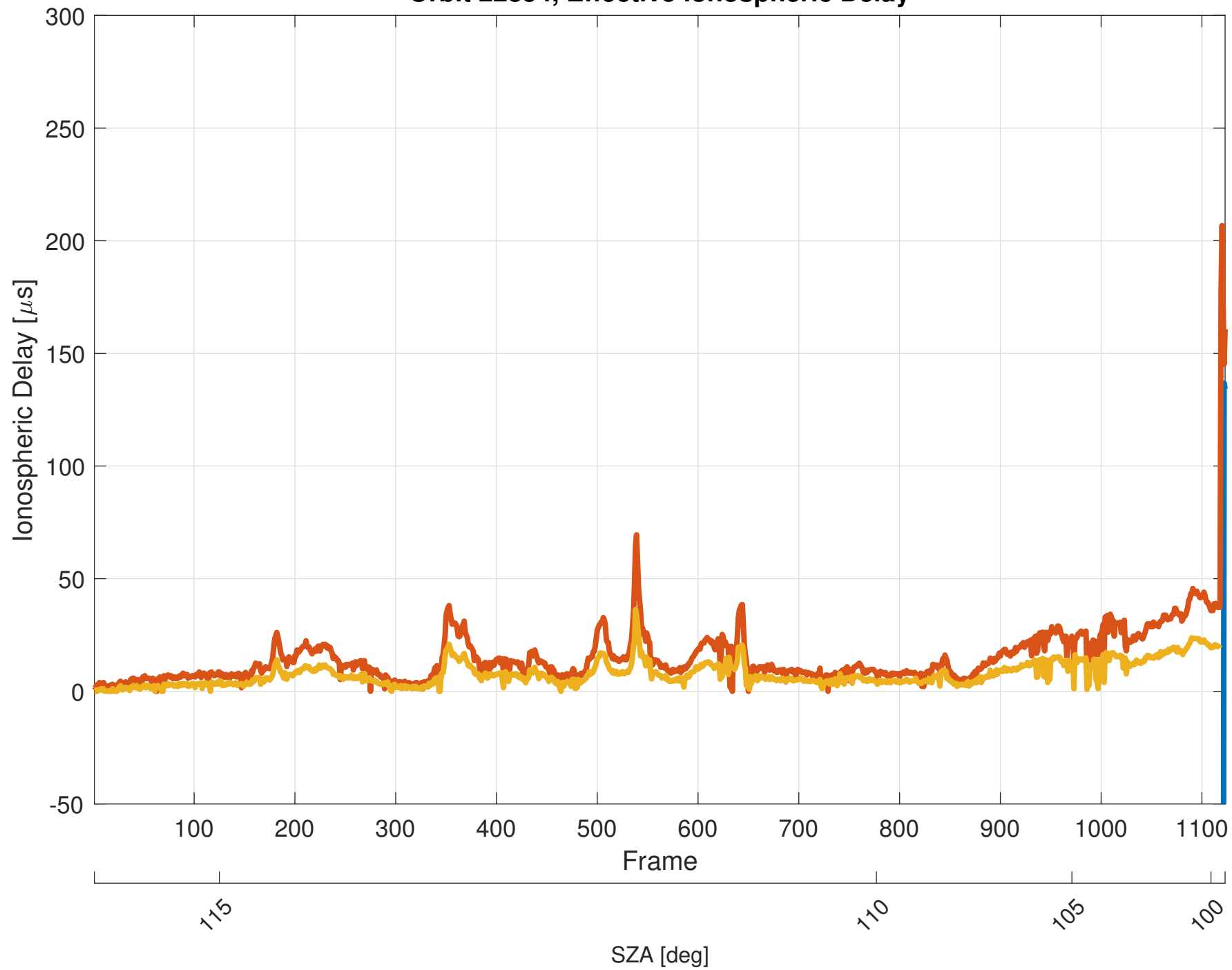
Orbit 22854, Effective Ionospheric Delay
