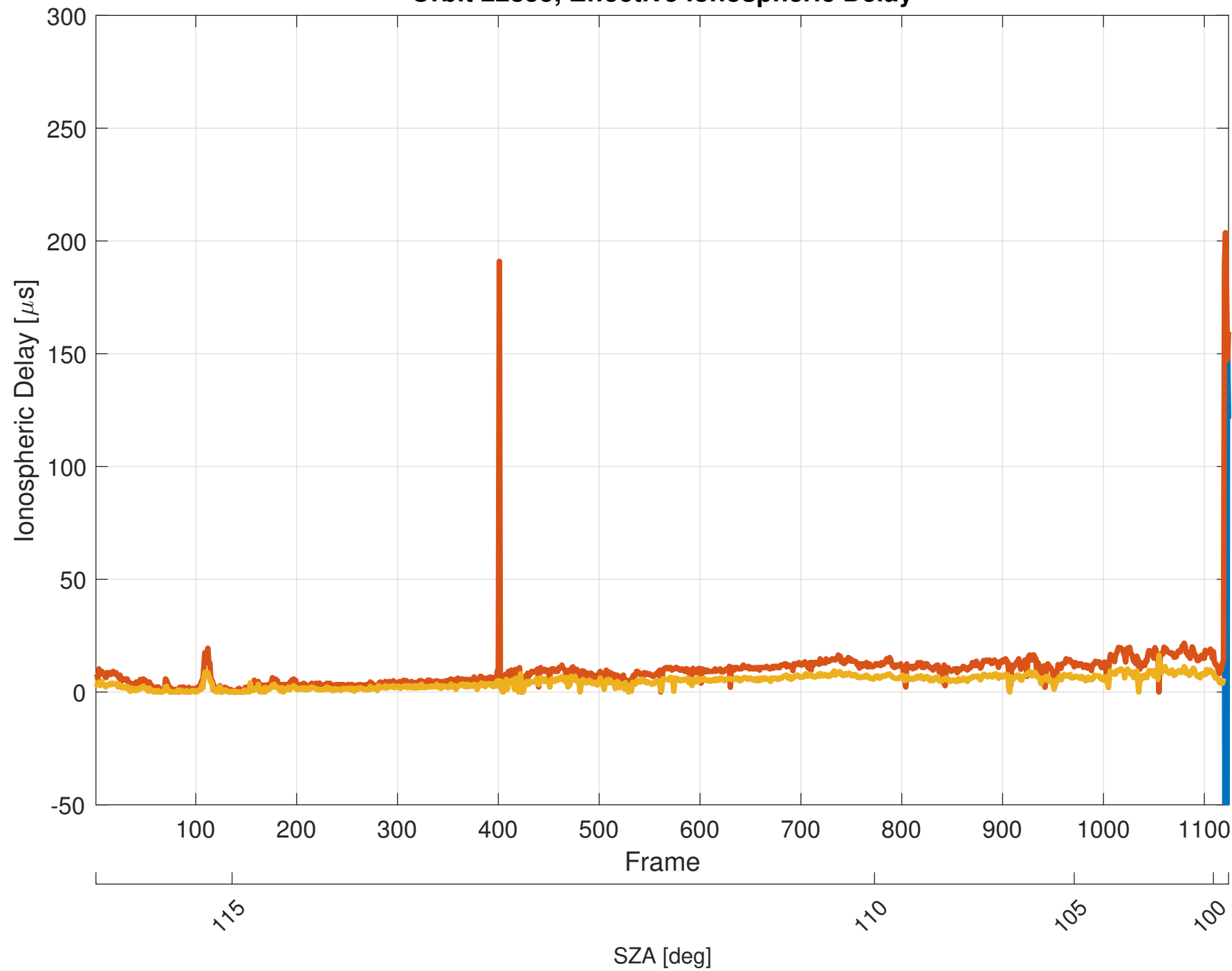
Orbit 22855, Effective Ionospheric Delay
