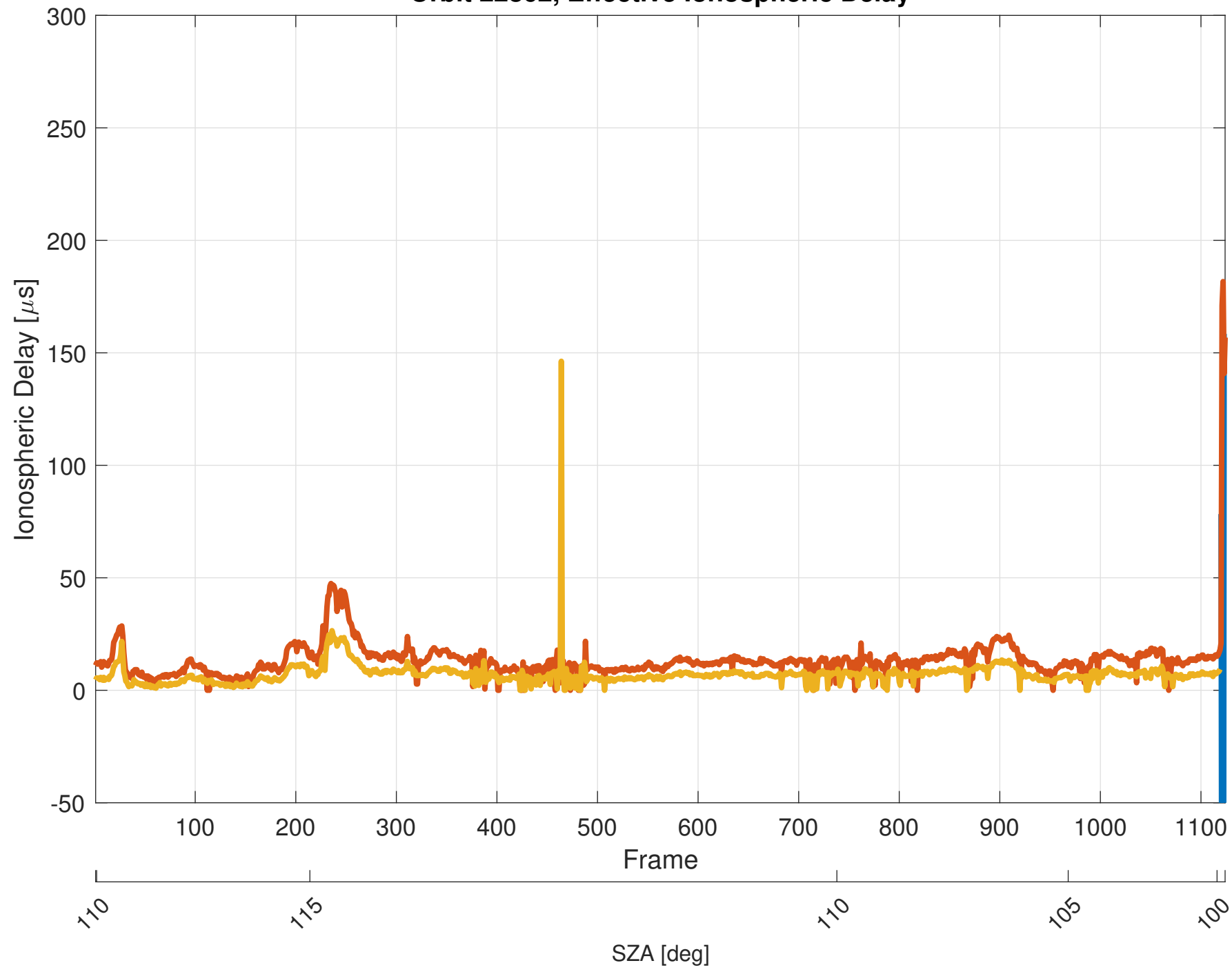
Orbit 22862, Effective Ionospheric Delay
