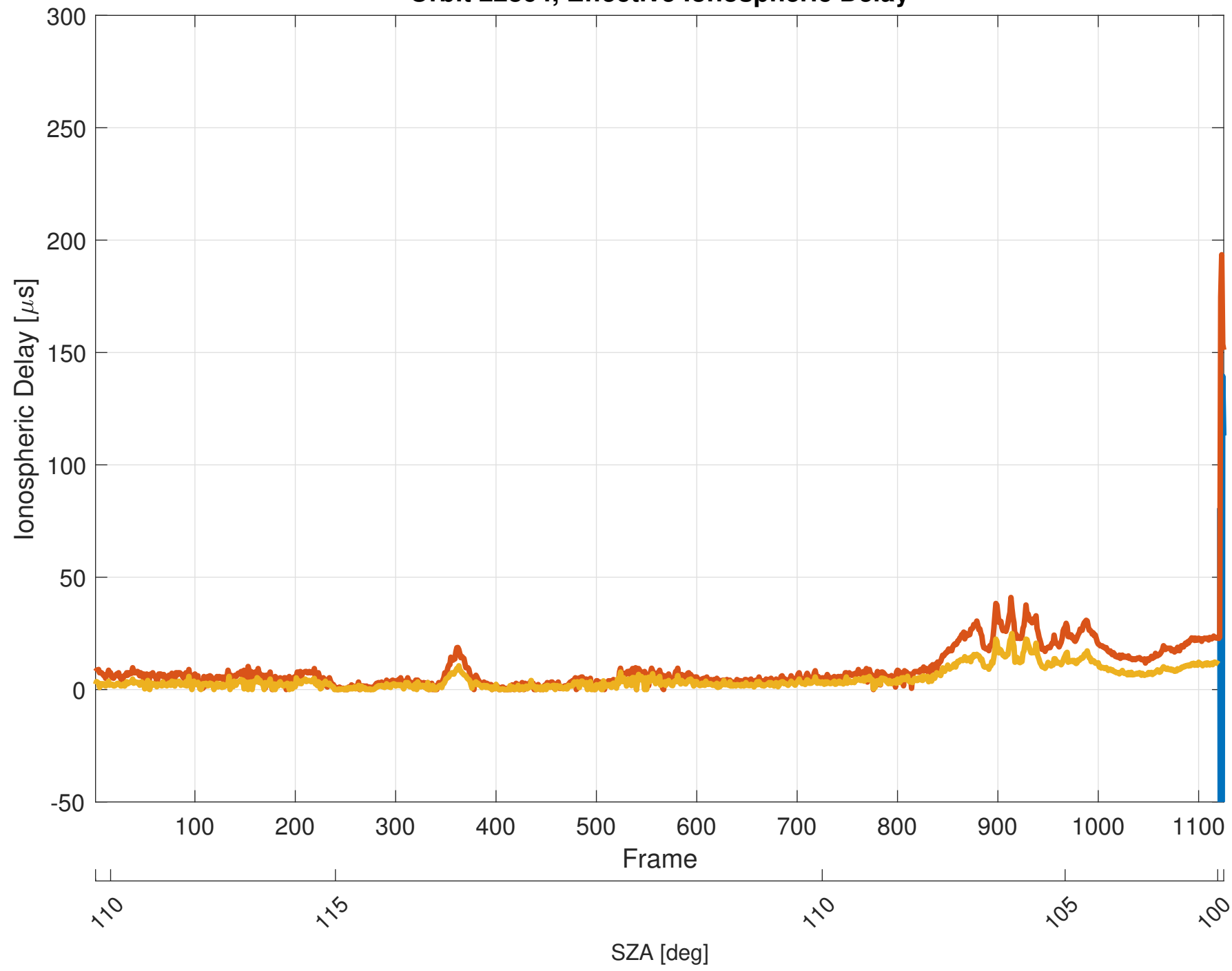
Orbit 22864, Effective Ionospheric Delay
