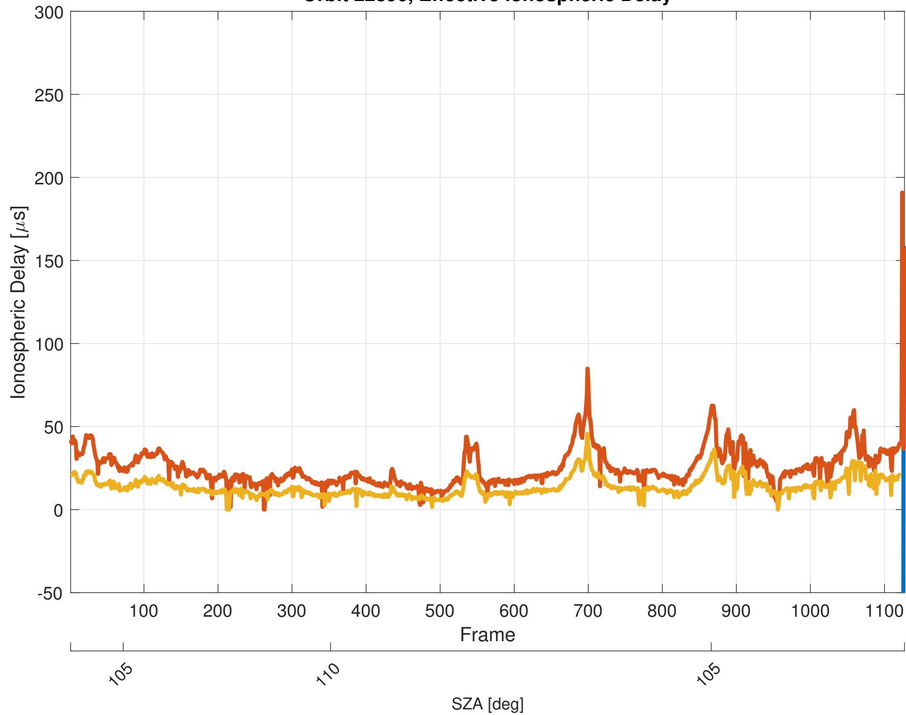
Orbit 22896, Effective Ionospheric Delay
