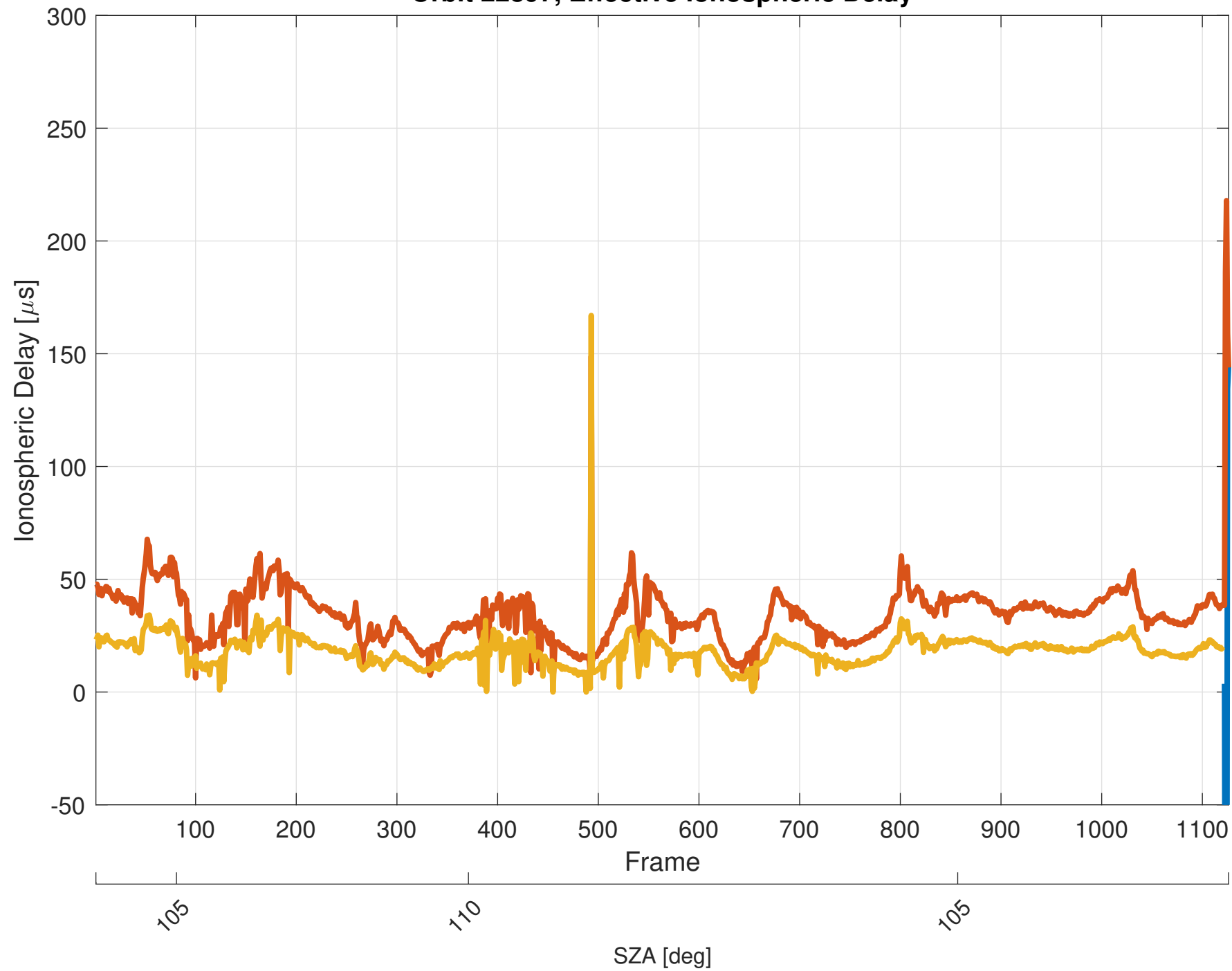
Orbit 22897, Effective Ionospheric Delay
