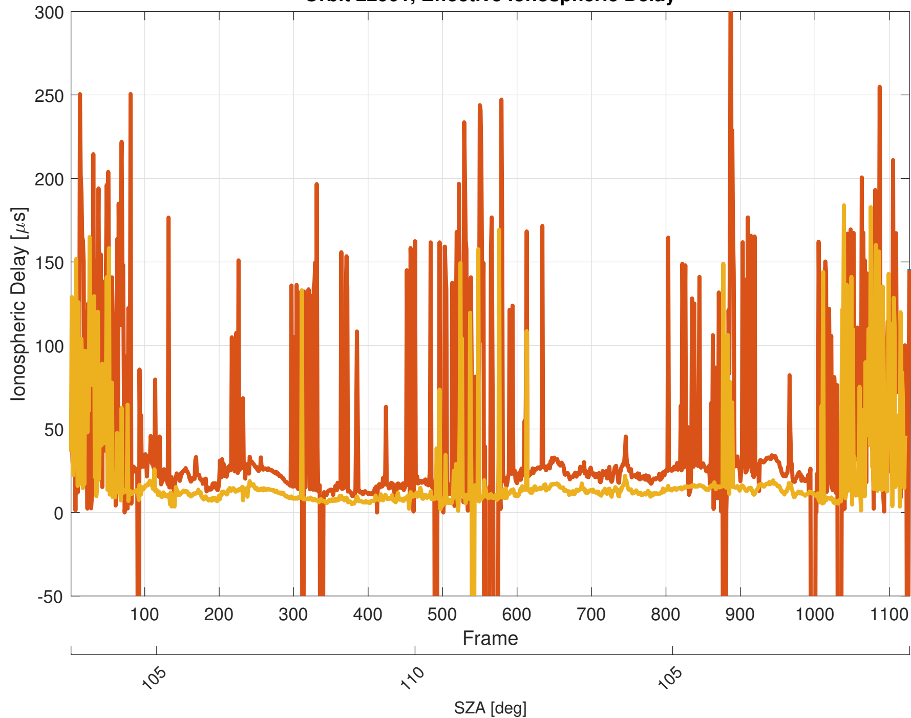
Orbit 22901, Effective Ionospheric Delay
