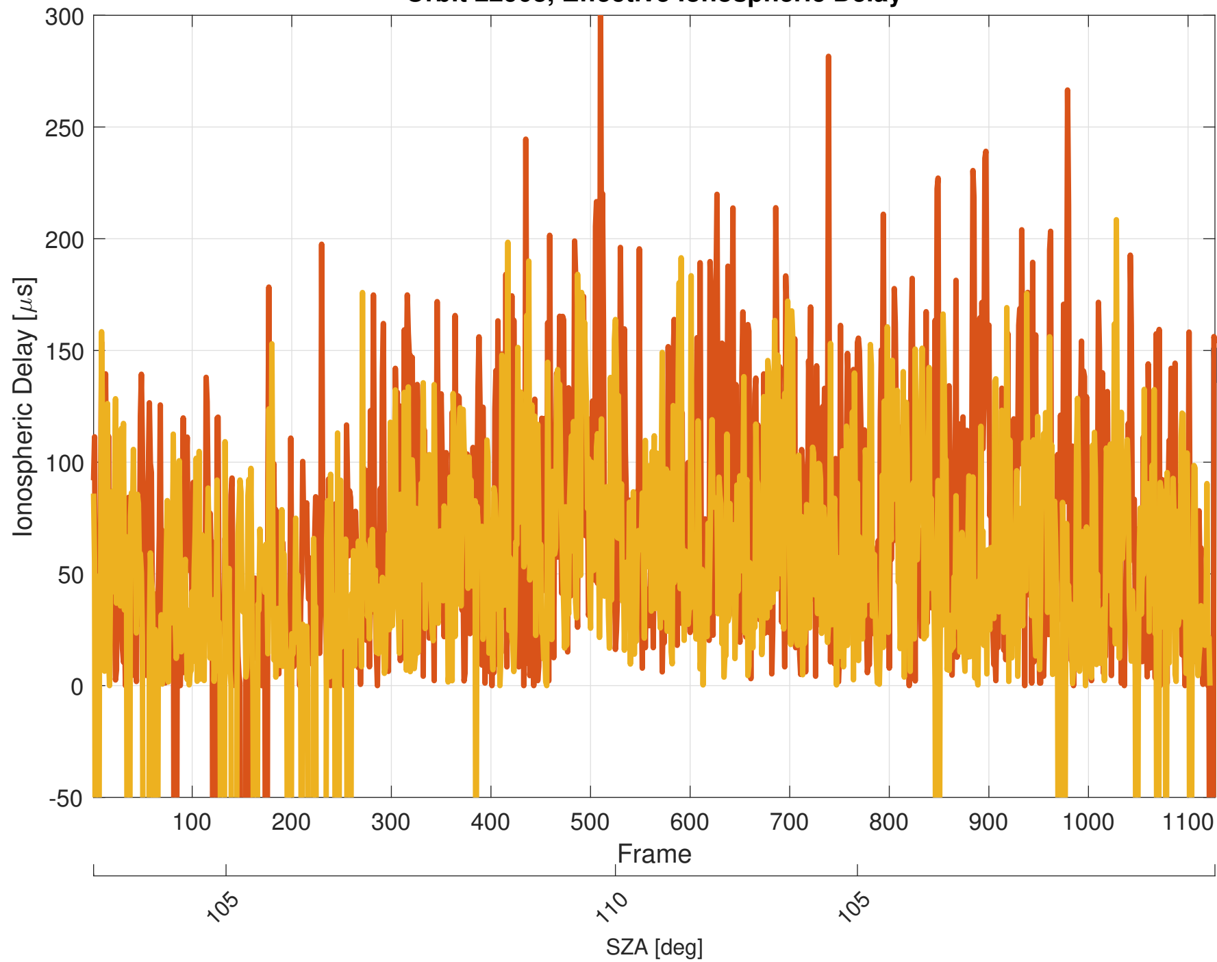
Orbit 22903, Effective Ionospheric Delay
