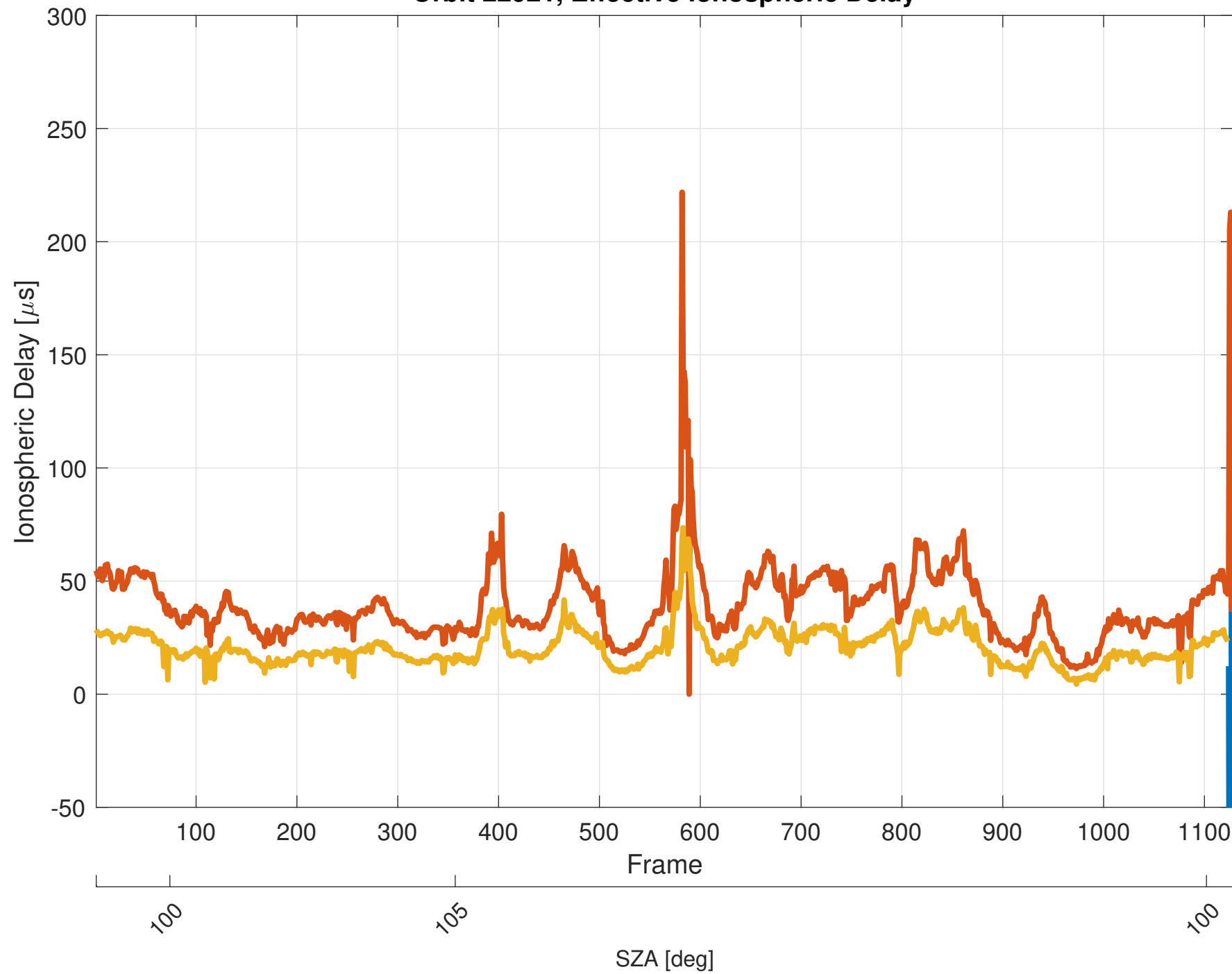
Orbit 22921, Effective Ionospheric Delay
